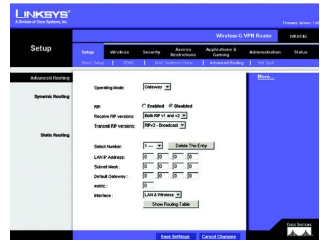
Figure 6-4: Password Tab
