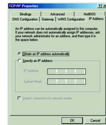
Figure 5-2: Connecting
