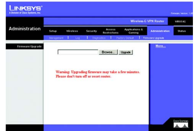
Figure C-1: Upgrade Firmware
