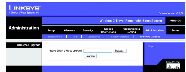
Figure C-1: Administration Tab - Firmware Upgrade
