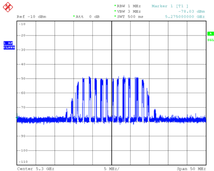
Waveform of EUT links up with Master
