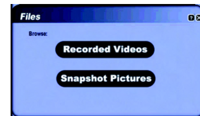
Figure 6-18: Files Screen
