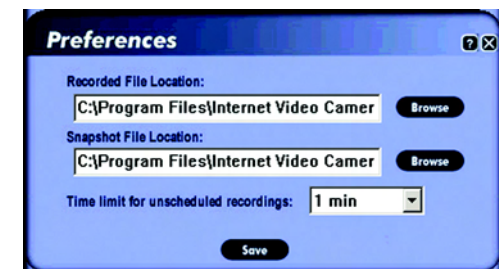
Figure 6-21: Preferences Screen
