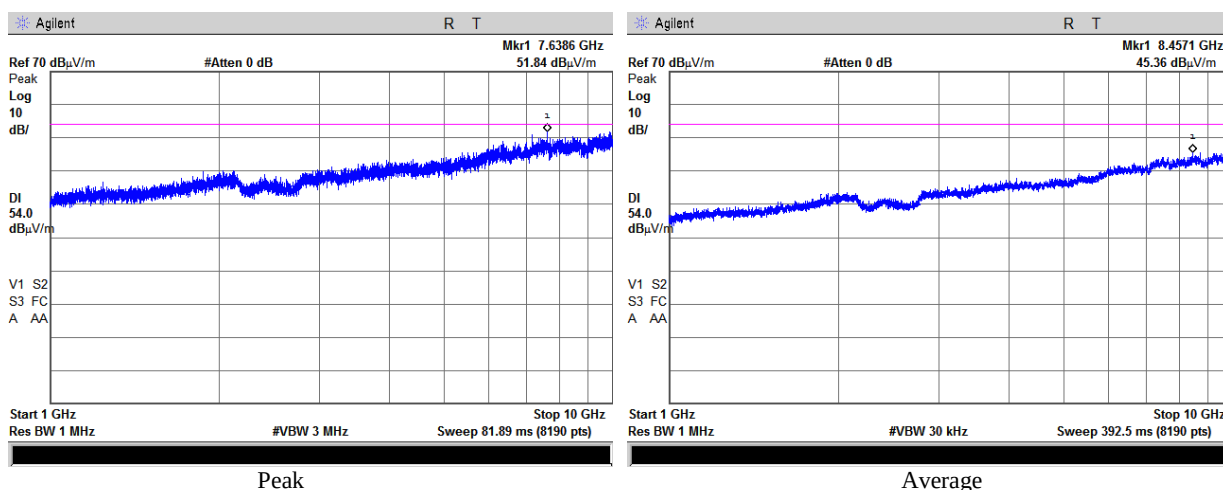
Plot 3.5.4 Emissions in restricted frequency bands test results, 1 – 10 GHz range, Horizontal, Fc = 2403 MHz, BW = 4.2 MHz, Bit Rate = 4 Mbps(with notch filter)
