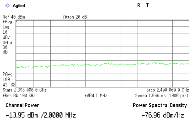
Plot 3.6.5 Band-Edge test results, BW = 4.2 MHz, Data rate = 4 Mbps, Fc = 2403 MHz
