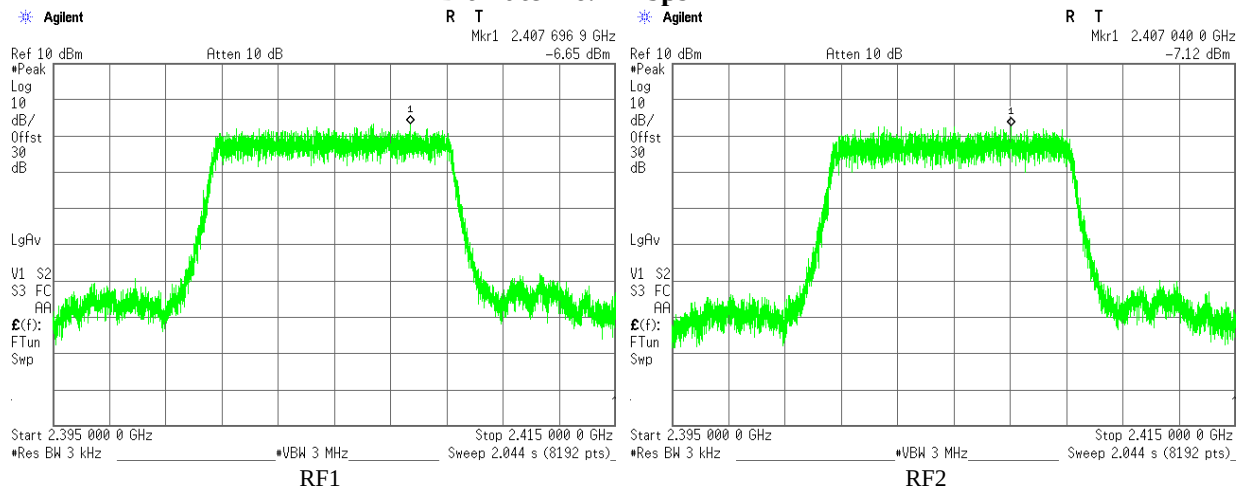
Plot 3.3.7 Maximum Power Spectral Density test results, F_c = 2405\text{MHz} , BW = 8.4\text{ MHz} , Bit Rate = 6.4 Mbps
