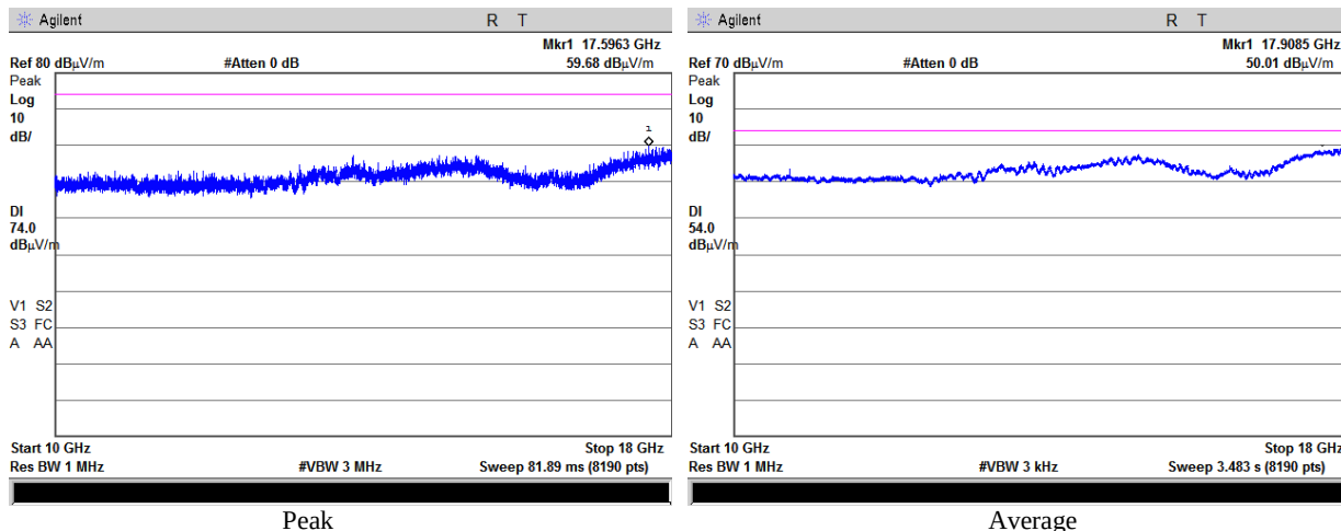
Plot 3.5.18 Emissions in restricted frequency bands test results, 10 – 18 GHz range, Horizontal, Fc = 2478 MHz, BW = 4.2 MHz, Bit Rate = 4 Mbps(with notch filter)
