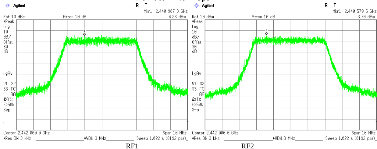
Plot 3.3.2 Maximum Power Spectral Density test results, F_c = 2442\text{MHz} , BW = 4.2\text{ MHz} , Bit Rate = 1.6 Mbps
