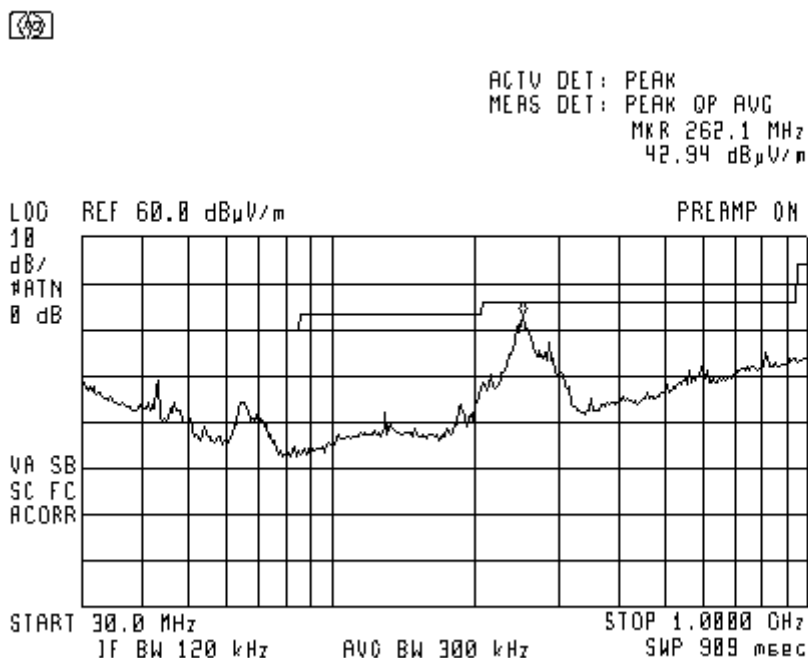
Plot 3.5.1 Emissions in restricted frequency bands test results, 30 MHz – 1 GHz range, Vertical polarization, Fc = 2403 MHz, BW = 4.2 MHz, Bit Rate = 4 Mbps (worst case for all modes)
