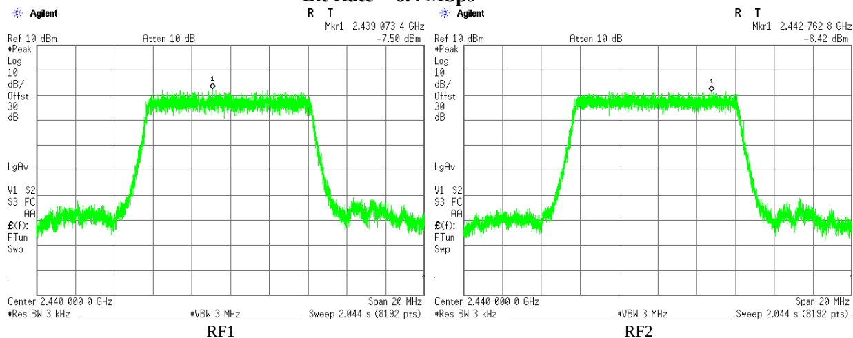
Plot 3.3.8 Maximum Power Spectral Density test results, F_c = 2440\text{MHz} , BW = 8.4\text{ MHz} , Bit Rate = 6.4 Mbps
