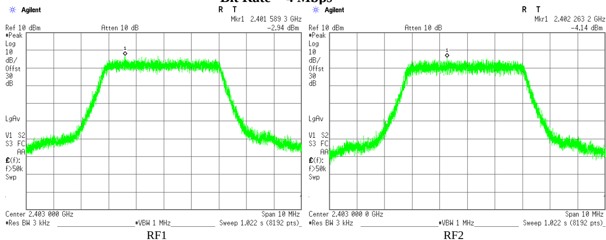
Plot 3.3.4 Maximum Power Spectral Density test results, F_c = 2403\text{MHz} , BW = 4.2\text{ MHz} , Bit Rate = 4 Mbps
