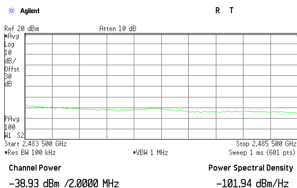
Plot 3.6.6 Band-Edge test results, BW = 4.2 MHz, Data rate = 4 Mbps, Fc = 2478 MHz
