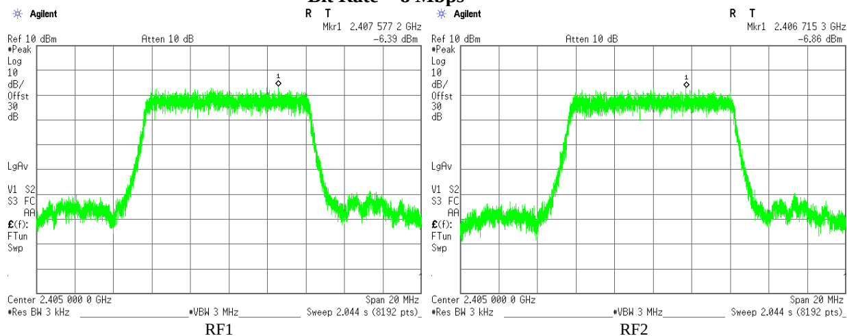
Plot 3.3.10 Maximum Power Spectral Density test results, F_c = 2405\text{MHz} , BW = 8.4\text{ MHz} , Bit Rate = 8 Mbps
