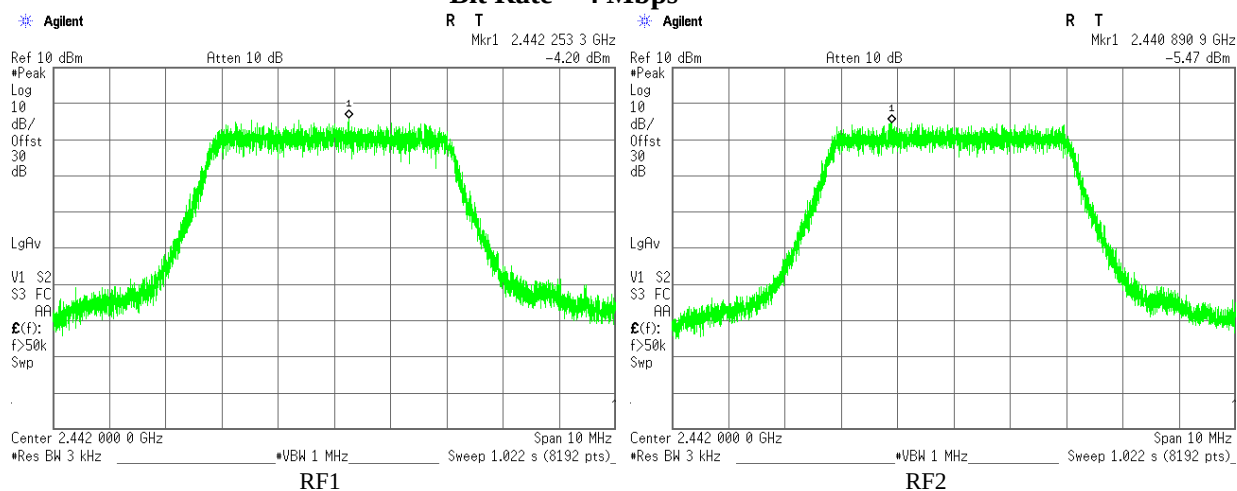
Plot 3.3.5 Maximum Power Spectral Density test results, F_c = 2442\text{MHz} , BW = 4.2\text{ MHz} , Bit Rate = 4 Mbps
