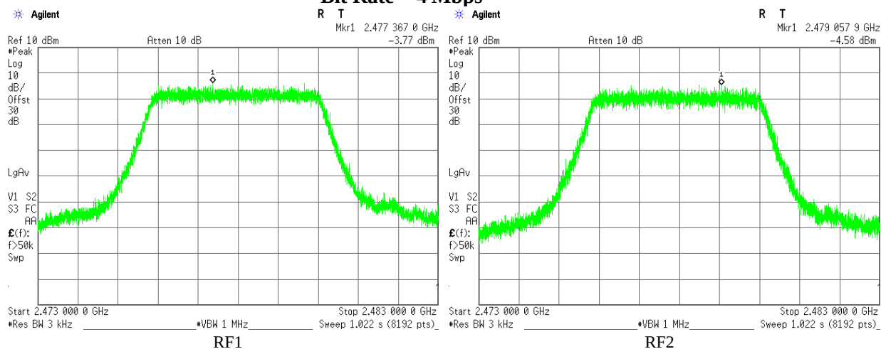
Plot 3.3.6 Maximum Power Spectral Density test results, F_c = 2478\text{MHz} , BW = 4.2\text{ MHz} , Bit Rate = 4 Mbps
