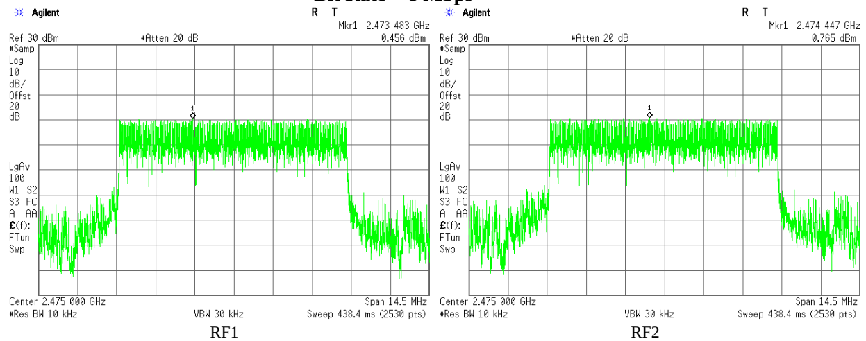
Plot 3.3.24 Maximum Power Spectral Density test results, F_c = 2475\text{MHz} , BW = 8.4\text{ MHz} , Bit Rate = 8 Mbps
