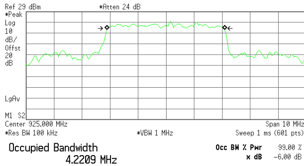
Plot 3.1.3 6 dB DTS Bandwidth, BW = 4.2 MHz, Bit rate = 3.2 Mbps, Fc = 925MHz
