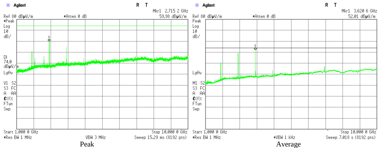
Plot 3.5.4 Emissions in restricted frequency bands test results, 1 – 10 GHz range, Horizontal, Fc = 905 MHz, BW = 4.2 MHz, Bit Rate = 3.2 Mbps
