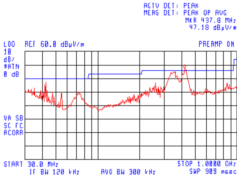
Plot 3.5.88 Emissions in restricted frequency bands test results, 30 MHz – 1 GHz range, Horizontal polarization, Fc = 2403 MHz, BW = 4.2 MHz, Bit Rate = 4 Mbps
