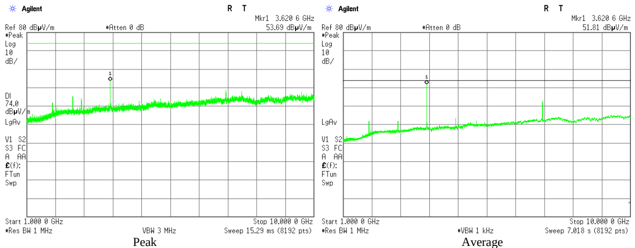
Plot 3.5.23 Emissions in restricted frequency bands test results, 1 – 10GHz range, Vertical, Fc = 915 MHz, BW = 8.4 MHz, Bit Rate = 8 Mbps
