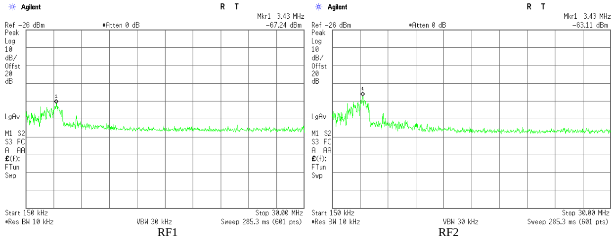
Plot 3.5.43 Emissions in restricted frequency bands test results, Conducted measurements, 150 kHz – 30 MHz, F_c = 905\text{ MHz} , BW = 4.2\text{ MHz} , Bit Rate = 4.0 Mbps
