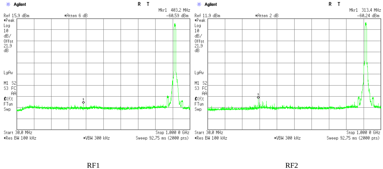
Plot 3.5.79 Emissions in restricted frequency bands test results, Conducted measurements, 30 MHz – 1000 MHz, Fc = 915 MHz, BW = 8.4 MHz, Bit Rate = 8 Mbps
