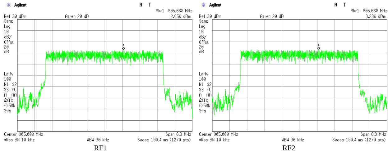
Plot 3.3.4 Maximum Power Spectral Density test results, F_c = 905\text{MHz} , BW = 4.2\text{ MHz} , Bit Rate = 4 Mbps
