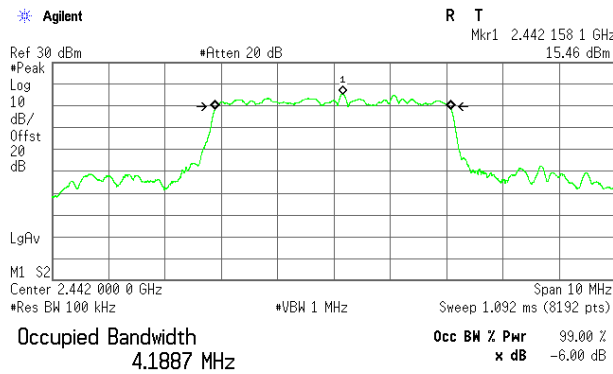
Plot 3.1.17 6 dB DTS Bandwidth, BW = 4.2 MHz, Bit rate = 4.0 Mbps, Fc = 2442
