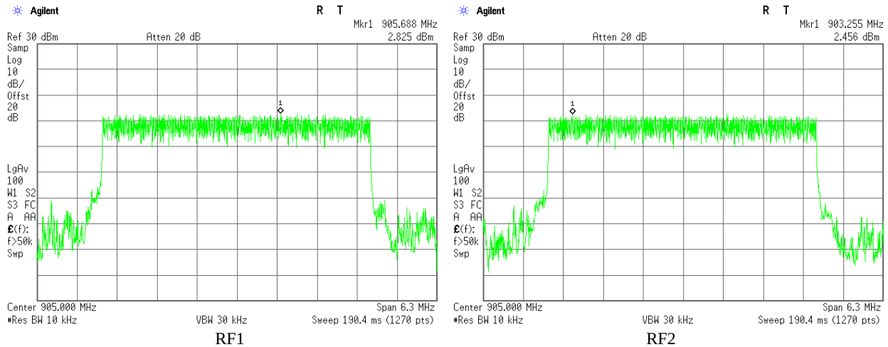
Plot 3.3.1 Maximum Power Spectral Density test results, F_c = 905\text{MHz} , BW = 4.2\text{ MHz} , Bit Rate = 3.2Mbps
