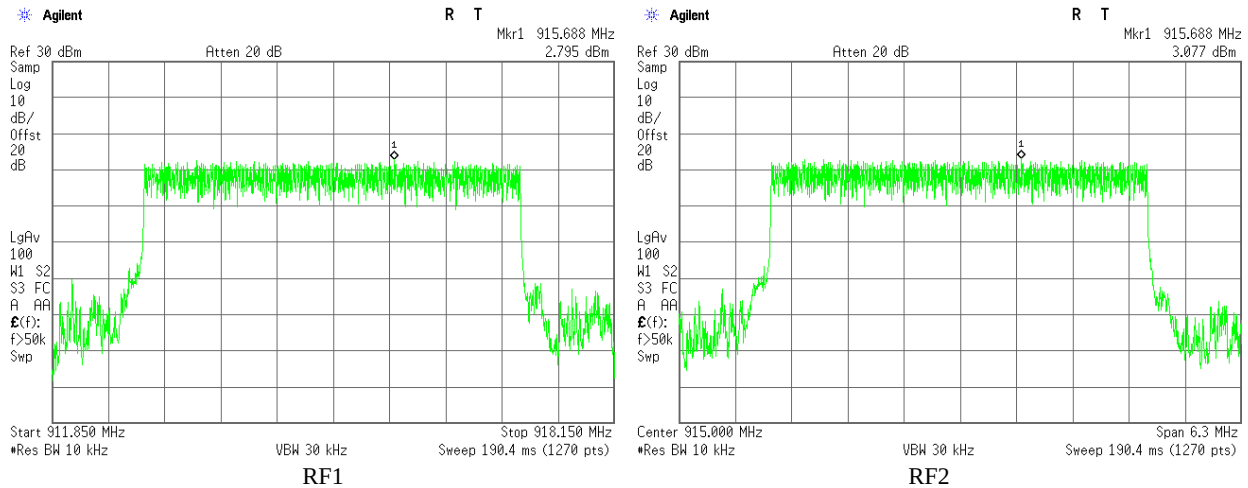
Plot 3.3.5 Maximum Power Spectral Density test results, F_c = 915\text{MHz} , BW = 4.2\text{ MHz} , Bit Rate = 4 Mbps
