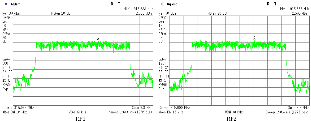
Plot 3.3.2 Maximum Power Spectral Density test results, F_c = 915\text{MHz} , BW = 4.2\text{ MHz} , Bit Rate = 3.2 Mbps
