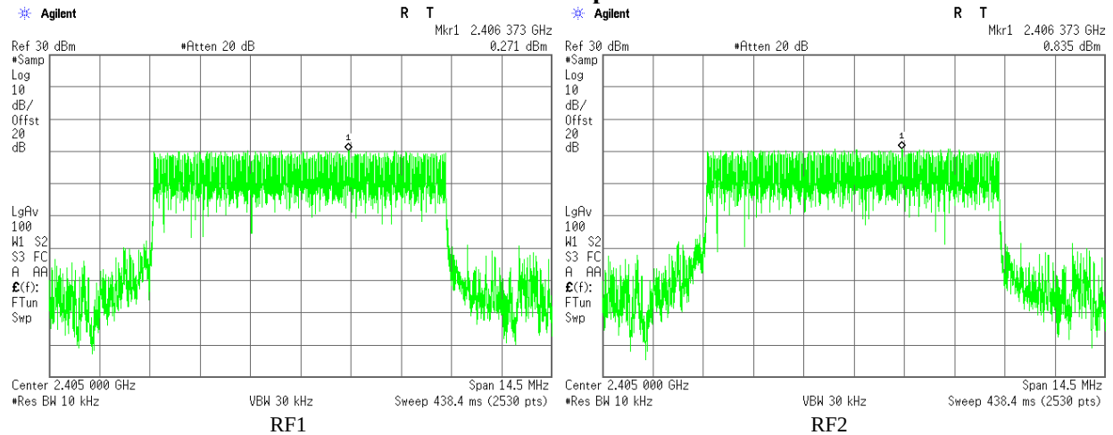
Plot 3.3.19 Maximum Power Spectral Density test results, F_c = 2405\text{MHz} , BW = 8.4\text{ MHz} , Bit Rate = 6.4 Mbps
