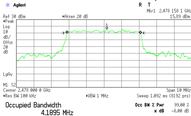
Plot 3.1.18 6 dB DTS Bandwidth, BW = 4.2 MHz, Bit rate = 4.0 Mbps, Fc = 2478MHz
