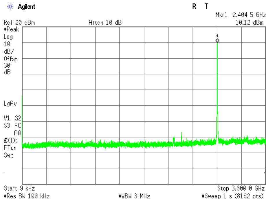
Plot 3.4.20 Unwanted Conducted Emissions into Non-Restricted Frequency Bands test results in 9 kHz – 3 GHz frequency range, F_c = 2403 MHz, BW = 4.2 MHz, Bit Rate = 4 MHz
