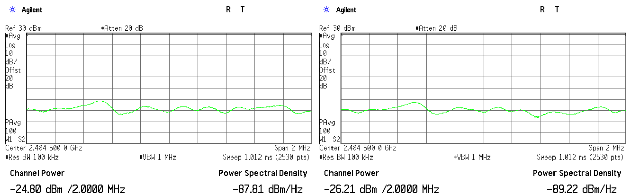
Plot 3.6.30 Band-Edge test results, BW = 8.4 MHz, Data rate = 6.4 Mbps, Fc = 2475 MHz
