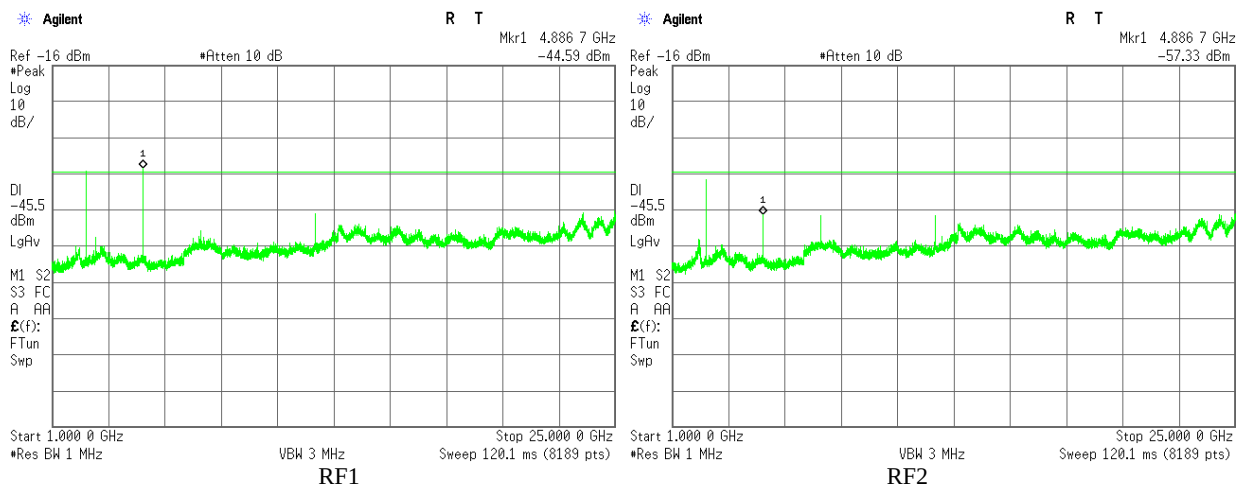
Plot 3.5.140 Emissions in restricted frequency bands test results, Conducted measurements, 1 GHz – 25 GHz, Fc = 2442 MHz, BW = 4.2 MHz, Bit Rate = 4 Mbps-(with notch filter)
