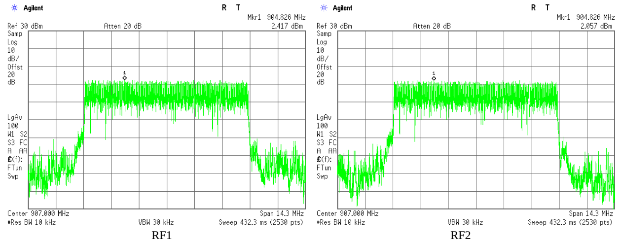
Plot 3.3.10 Maximum Power Spectral Density test results, F_c = 907\text{MHz} , BW = 8.4\text{ MHz} , Bit Rate = 8 Mbps
