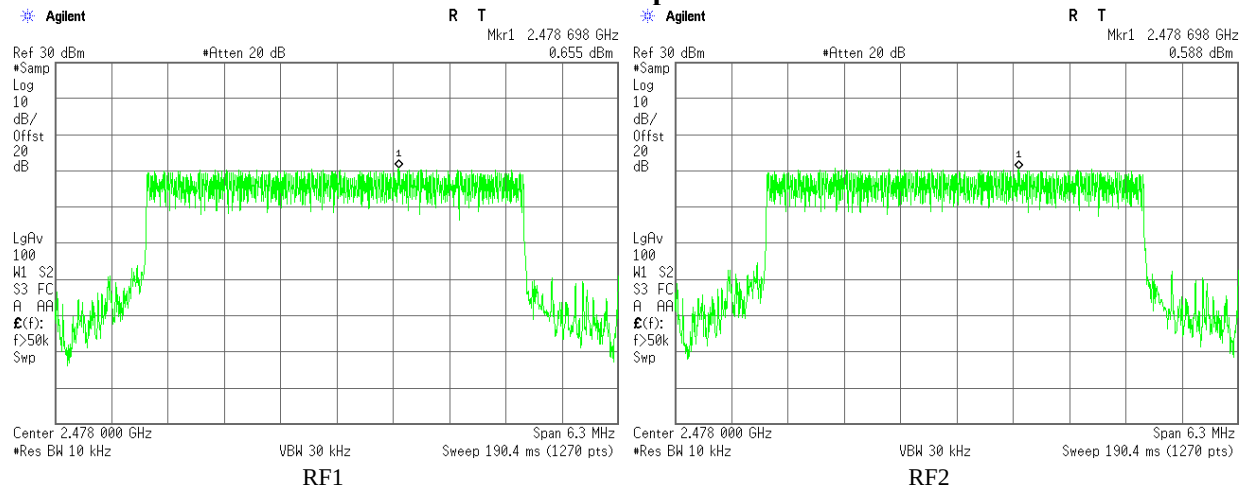
Plot 3.3.18 Maximum Power Spectral Density test results, F_c = 2478\text{MHz} , BW = 4.2\text{ MHz} , Bit Rate = 4 Mbps
