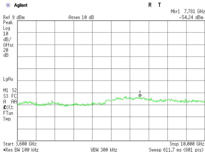
Plot 3.4.18 Unwanted Conducted Emissions into Non-Restricted Frequency Bands test results in 3.6 GHz – 10 GHz frequency range, F_c = 923\text{ MHz} , BW = 8.4\text{ MHz} , Bit Rate = 8 MHz
