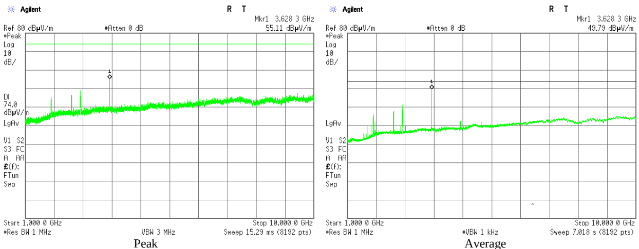
Plot 3.5.22 Emissions in restricted frequency bands test results, 1 – 10 GHz range, Horizontal, F_c = 907 MHz, BW = 8.4 MHz, Bit Rate = 8 Mbps
