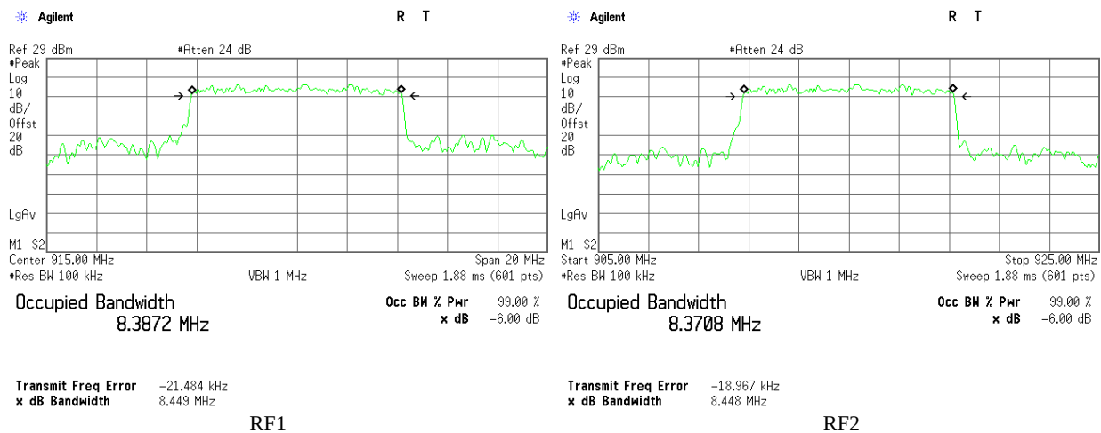
Plot 3.1.8 6 dB DTS Bandwidth, BW = 8.4 MHz, Bit rate = 6.4 Mbps, Fc = 915 MHz
