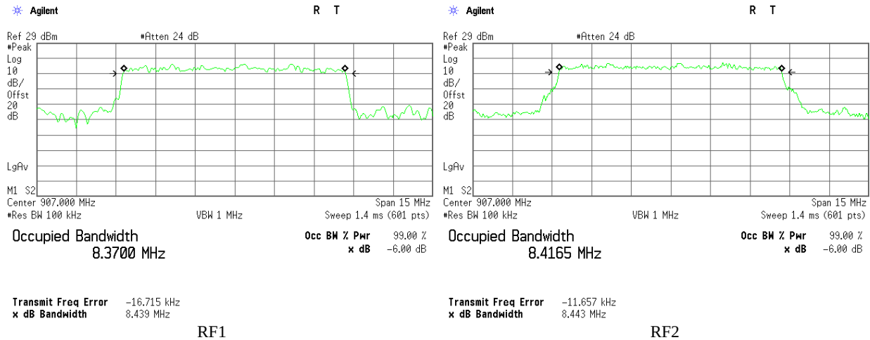
Plot 3.1.7 6 dB DTS Bandwidth, BW = 8.4 MHz, Bit rate = 6.4 Mbps, Fc = 907 MHz
