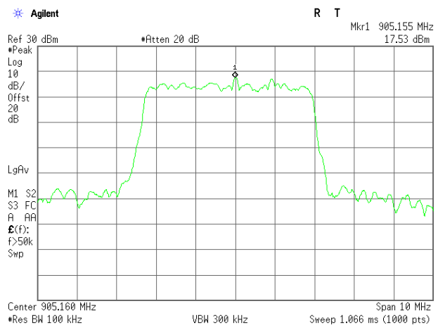
Plot 3.6.2 Band-Edge test results, Fundamental Emission Reference Level, BW = 4.2 MHz, Data rate = 4 Mbps, Fc = 905 MHz
