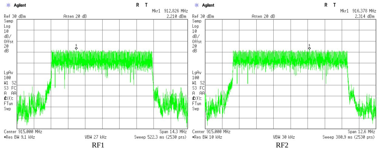
Plot 3.3.8 Maximum Power Spectral Density test results, F_c = 915\text{MHz} , BW = 8.4\text{ MHz} , Bit Rate = 6.4 Mbps
