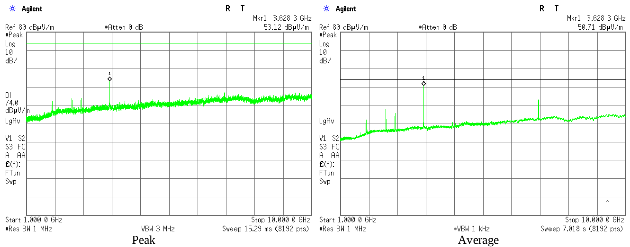
Plot 3.5.21 Emissions in restricted frequency bands test results, 1 – 10 GHz range, Vertical, F_c = 907 MHz, BW = 8.4 MHz, Bit Rate = 8 Mbps
