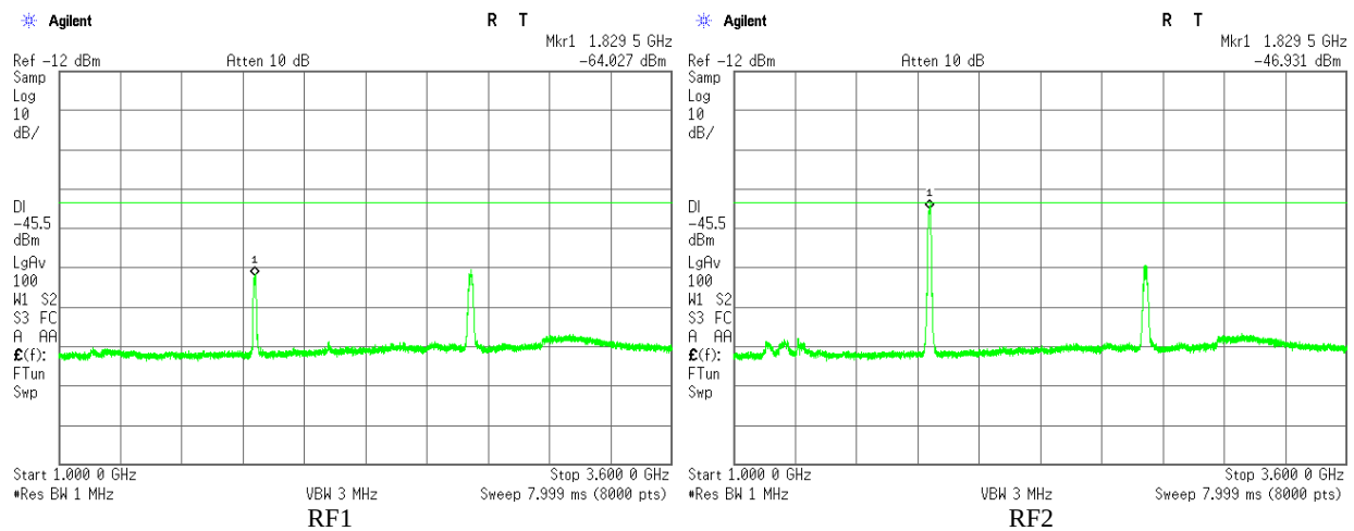
Plot 3.5.80 Emissions in restricted frequency bands test results, Conducted measurements, 1 GHz – 3.6 GHz, Fc = 915 MHz, BW = 8.4 MHz, Bit Rate = 8 Mbps
