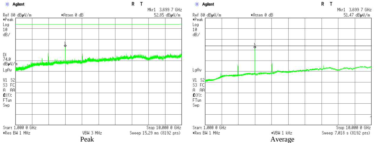
Plot 3.5.7 Emissions in restricted frequency bands test results, 1 – 10 GHz range, Vertical, Fc = 925 MHz, BW = 4.2 MHz, Bit Rate = 3.2 Mbps
