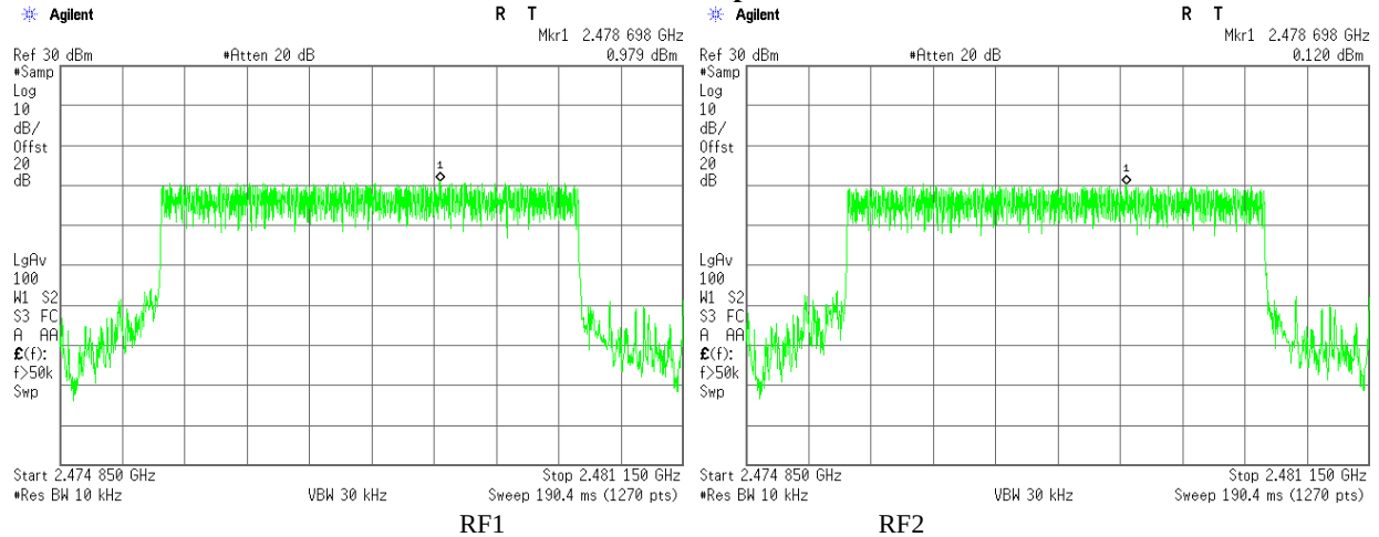
Plot 3.3.15 Maximum Power Spectral Density test results, F_c = 2478\text{MHz} , BW = 4.2\text{ MHz} , Bit Rate = 3.2 Mbps
