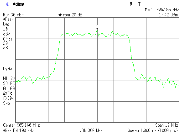
Plot 3.6.1 Band-Edge test results, Fundamental Emission Reference Level, BW = 4.2 MHz, Data rate = 3.2 Mbps, Fc = 905 MHz
