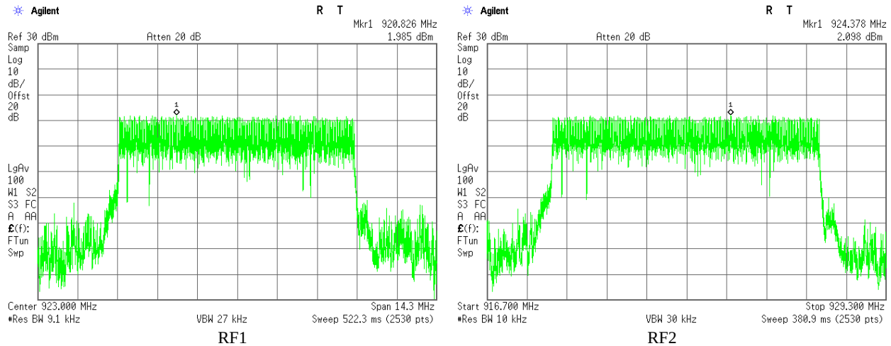
Plot 4.3.9 Maximum Power Spectral Density test results, F_c = 923\text{MHz} , BW = 8.4\text{ MHz} , Bit Rate = 6.4 Mbps
