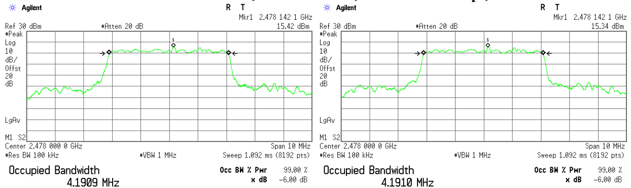
Plot 3.1.15 6 dB DTS Bandwidth, BW = 4.2 MHz, Bit rate = 3.2 Mbps, Fc = 2478MHz
