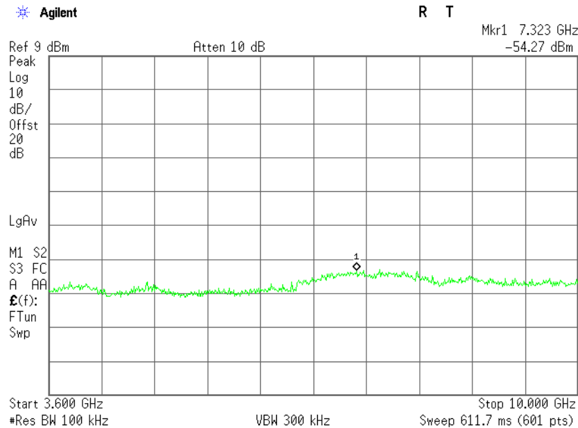
Plot 3.4.15 Unwanted Conducted Emissions into Non-Restricted Frequency Bands test results in 3.6 GHz – 10 GHz frequency range, F_c = 915\text{ MHz} , BW = 8.4\text{ MHz} , Bit Rate = 8 MHz
