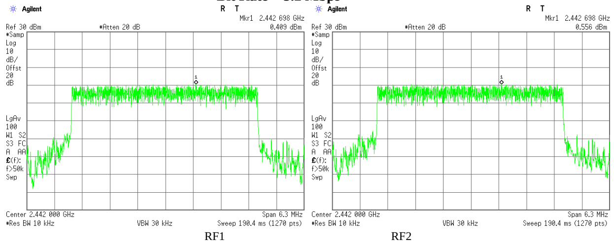
Plot 3.3.14 Maximum Power Spectral Density test results, F_c = 2442\text{MHz} , BW = 4.2\text{ MHz} , Bit Rate = 3.2 Mbps
