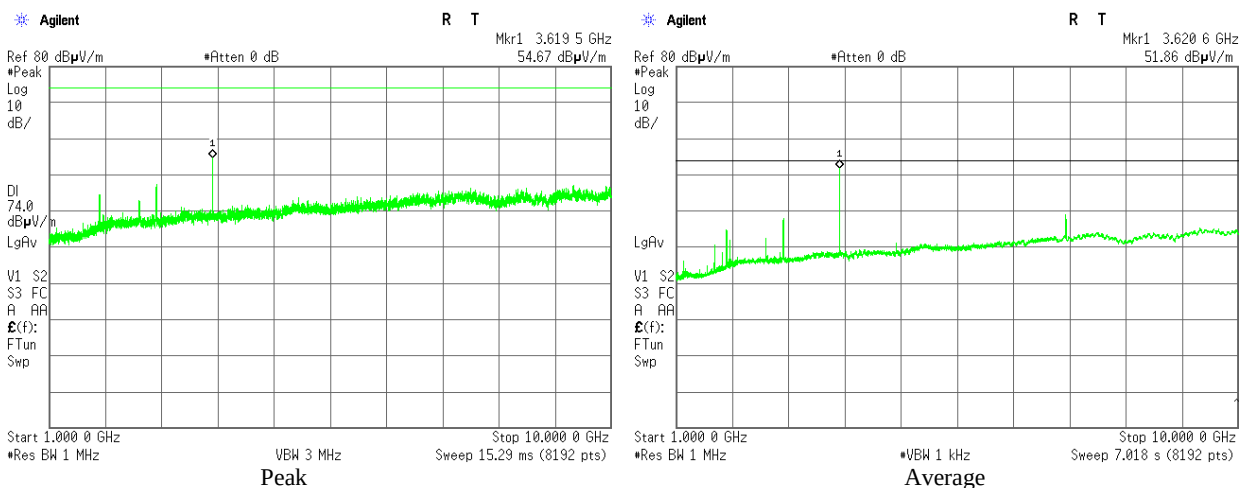
Plot 3.5.24 Emissions in restricted frequency bands test results, 1 – 10 GHz range, Horizontal, Fc = 915 MHz, BW = 8.4 MHz, Bit Rate = 8 Mbps
