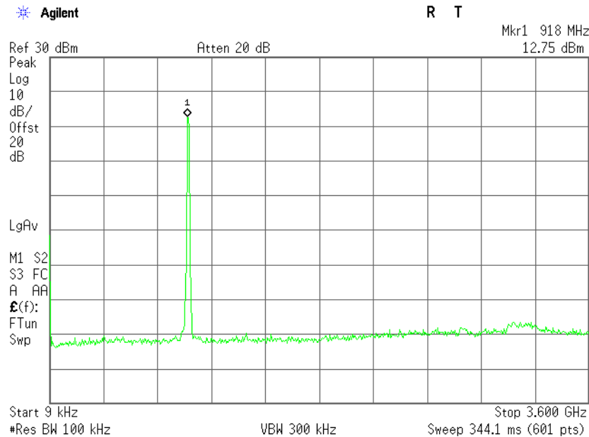
Plot 3.4.17 Unwanted Conducted Emissions into Non-Restricted Frequency Bands test results in 9 kHz – 3.6 GHz frequency range, F_c = 923\text{ MHz} , BW = 8.4\text{ MHz} , Bit Rate = 8 MHz
