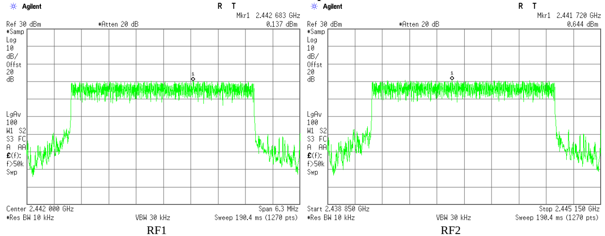
Plot 3.3.17 Maximum Power Spectral Density test results, F_c = 2442\text{MHz} , BW = 4.2\text{ MHz} , Bit Rate = 4 Mbps
