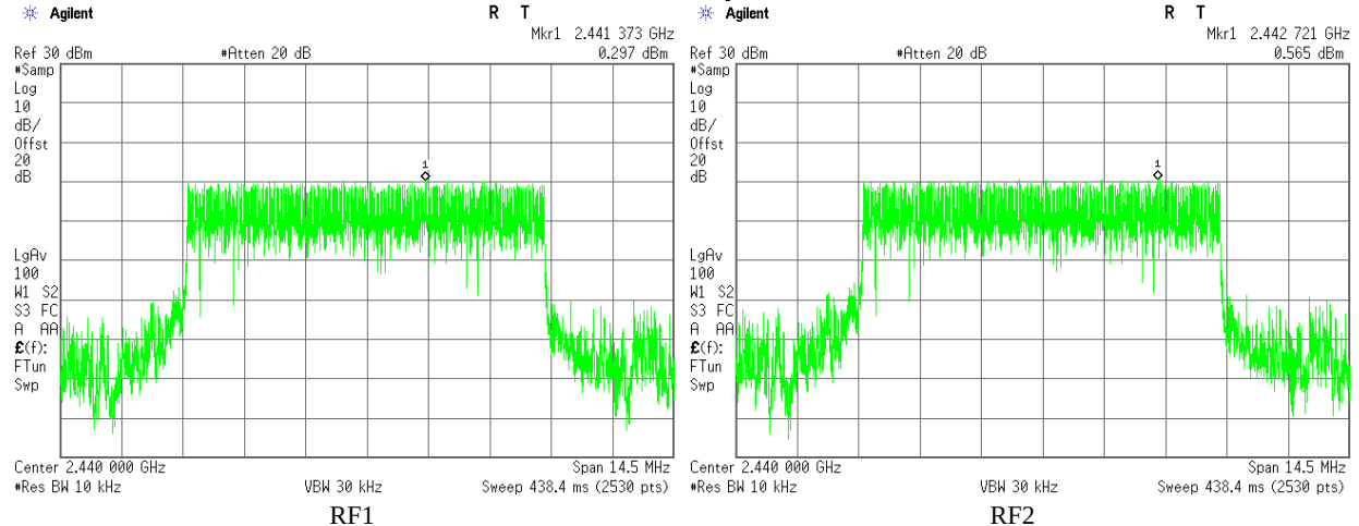
Plot 3.3.20 Maximum Power Spectral Density test results, F_c = 2440\text{MHz} , BW = 8.4\text{ MHz} , Bit Rate = 6.4 Mbps
