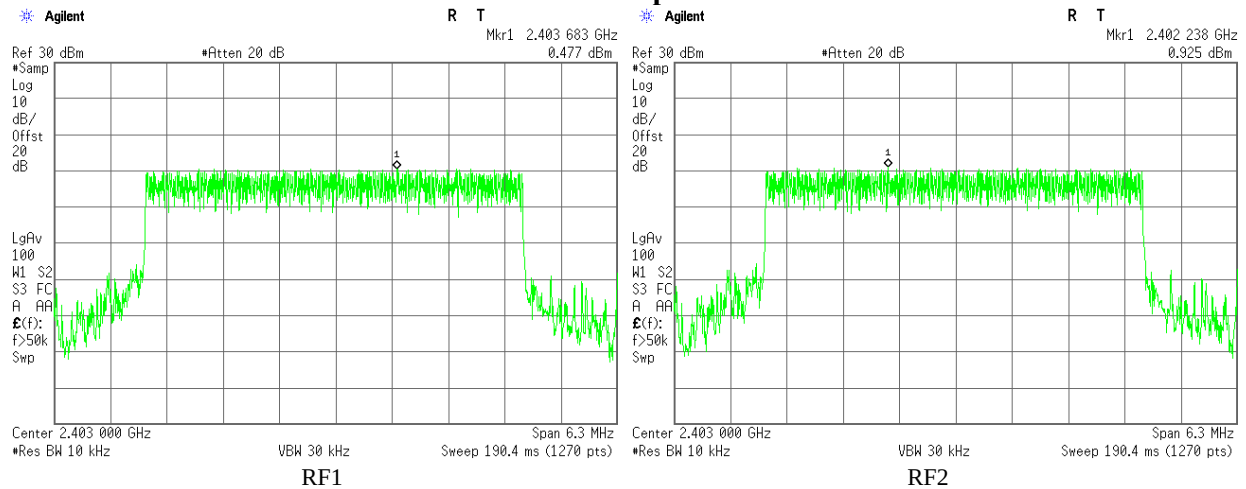
Plot 3.3.16 Maximum Power Spectral Density test results, F_c = 2403\text{MHz} , BW = 4.2\text{ MHz} , Bit Rate = 4 Mbps
