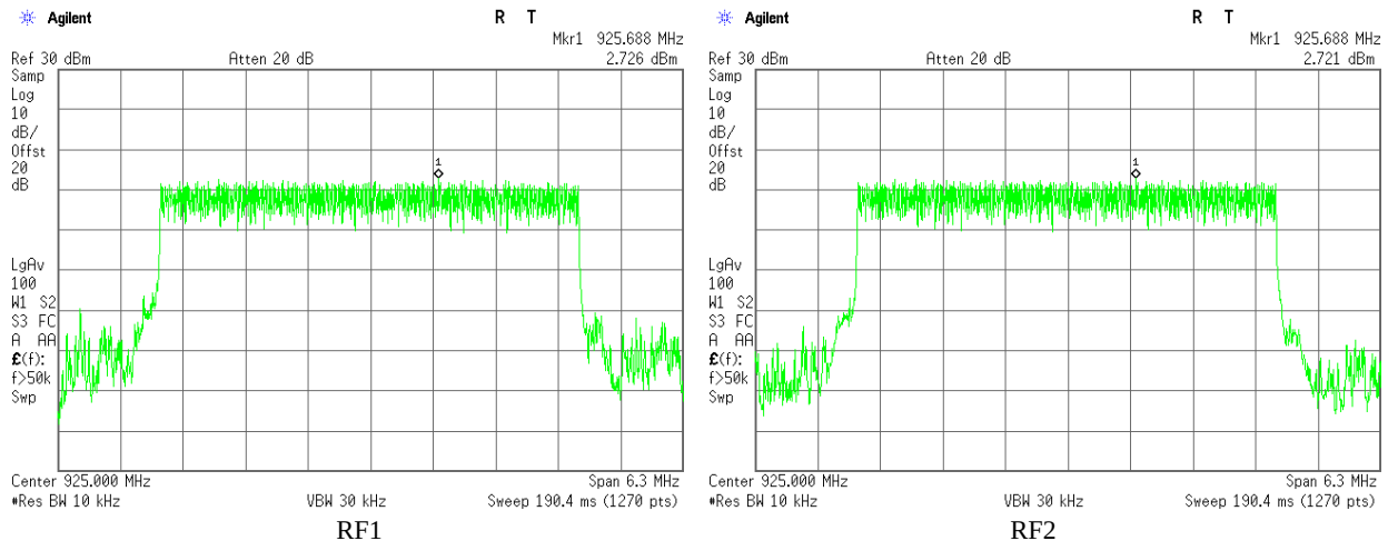
Plot 3.3.6 Maximum Power Spectral Density test results, F_c = 925\text{MHz} , BW = 4.2\text{ MHz} , Bit Rate = 4 Mbps
