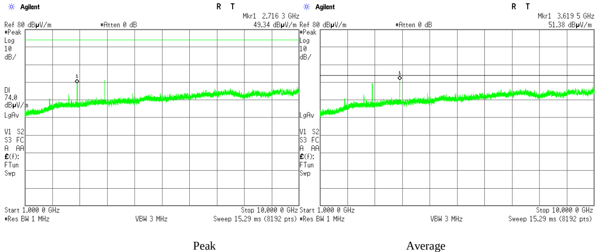
Plot 3.5.3 Emissions in restricted frequency bands test results, 1 – 10 GHz range, Vertical, Fc = 905 MHz, BW = 4.2 MHz, Bit Rate = 3.2 Mbps
