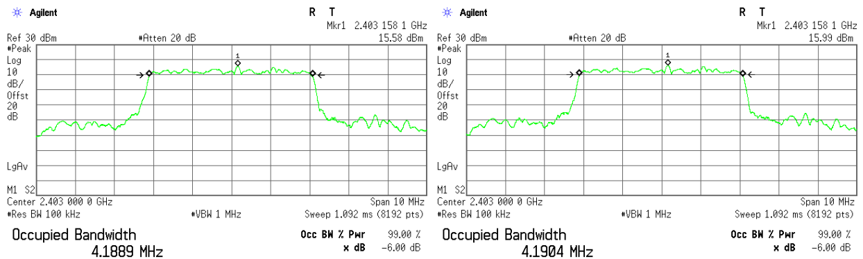
Plot 3.1.16 6 dB DTS Bandwidth, BW = 4.2 MHz, Bit rate = 4.0 Mbps, Fc = 2403MHz
