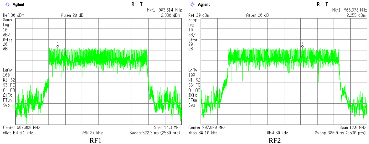
Plot 3.3.7 Maximum Power Spectral Density test results, F_c = 907\text{MHz} , BW = 8.4\text{ MHz} , Bit Rate = 6.4 Mbps
