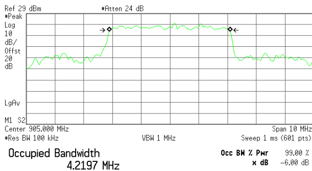
Plot 3.1.4 6 dB DTS Bandwidth, BW = 4.2 MHz, Bit rate = 4.0 Mbps, Fc = 905MHz
