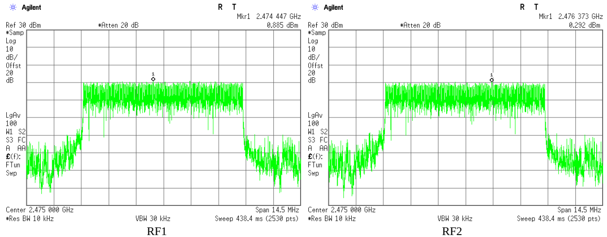
Plot 4.3.21 Maximum Power Spectral Density test results, F_c = 2475\text{MHz} , BW = 8.4\text{ MHz} , Bit Rate = 6.4 Mbps
