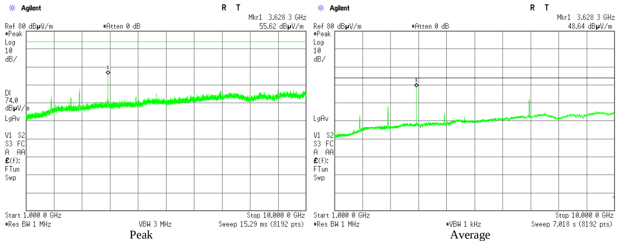
Plot 3.5.15 Emissions in restricted frequency bands test results, 1 – 10 GHz range, Vertical, F_c = 907 \text{ MHz} , BW = 8.4 \text{ MHz} , Bit Rate = 6.4 Mbps
