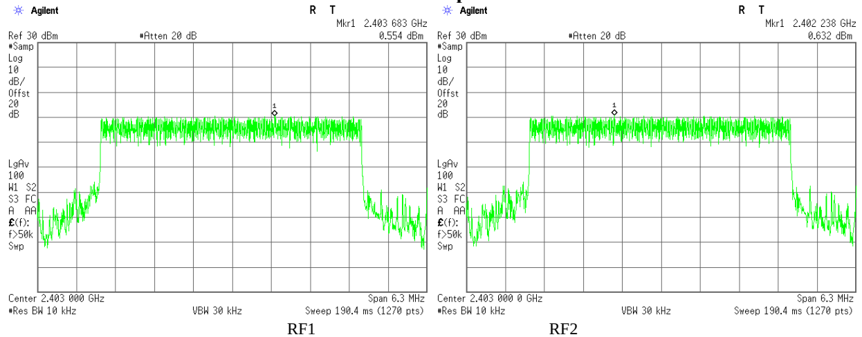
Plot 3.3.13 Maximum Power Spectral Density test results, F_c = 2403\text{MHz} , BW = 4.2\text{ MHz} , Bit Rate = 3.2Mbps
