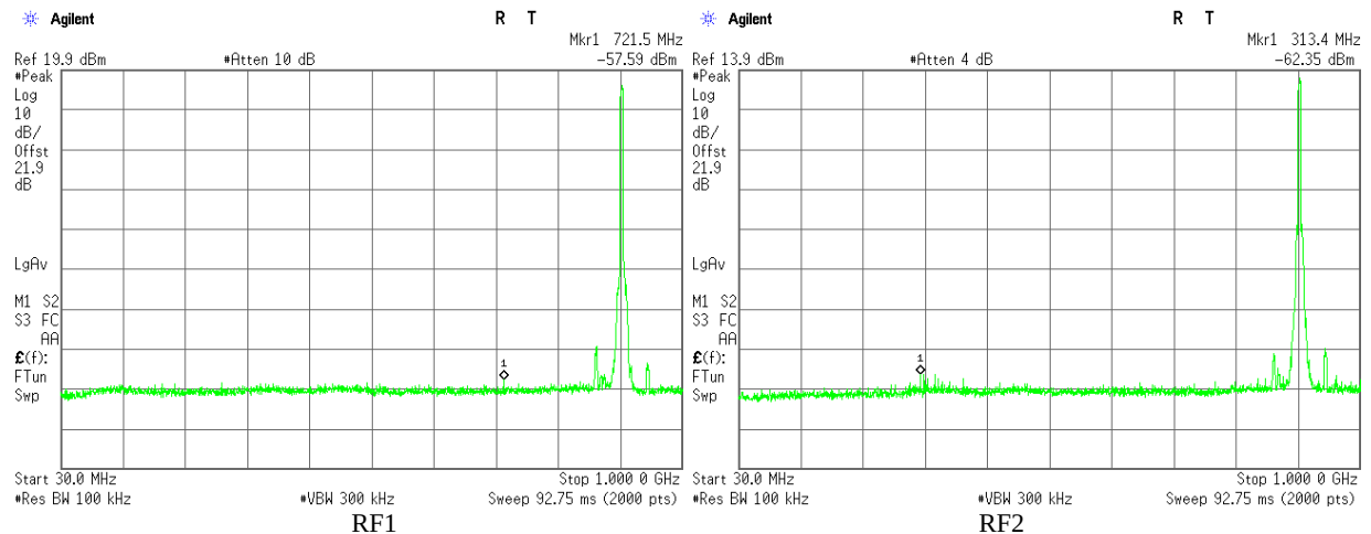
Plot 3.5.44 Emissions in restricted frequency bands test results, Conducted measurements, 30 MHz – 1000 MHz, F_c = 905\text{ MHz} , BW = 4.2\text{ MHz} , Bit Rate = 4 Mbps
