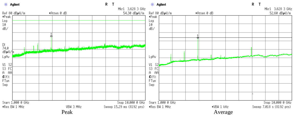
Plot 3.5.16 Emissions in restricted frequency bands test results, 1 – 10 GHz range, Horizontal, F_c = 907 \text{ MHz} , BW = 8.4 \text{ MHz} , Bit Rate = 6.4 Mbps
