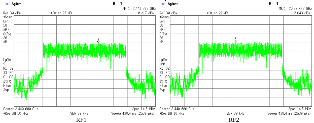
Plot 3.3.23 Maximum Power Spectral Density test results, F_c = 2440\text{MHz} , BW = 8.4\text{ MHz} , Bit Rate = 8 Mbps
