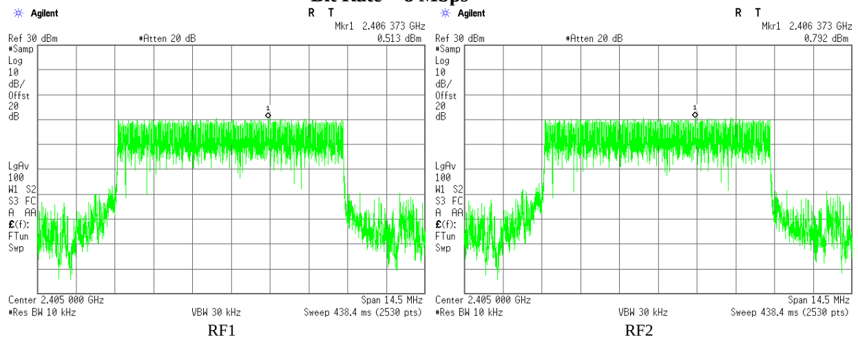
Plot 3.3.22 Maximum Power Spectral Density test results, F_c = 2405\text{MHz} , BW = 8.4\text{ MHz} , Bit Rate = 8 Mbps
