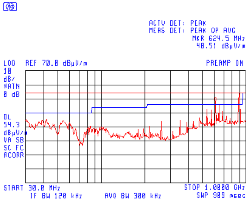
Plot 3.5.1 Emissions in restricted frequency bands test results, 30 MHz – 1 GHz range, Vertical polarization, Fc = 915 MHz, BW = 8.4 MHz, Bit Rate = 6.4 Mbps
