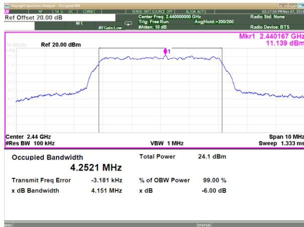
Plot 3.1.2 6 dB DTS Bandwidth, BW = 4.2 MHz, Bit rate = 1.6 Mbps, Fc = 2440MHz
