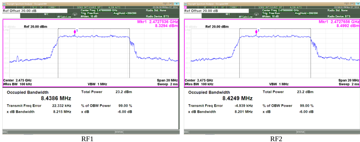
Plot 3.1.12 6 dB DTS Bandwidth, BW = 8.4 MHz, Bit rate = 8.0 Mbps, Fc = 2475 MHz
