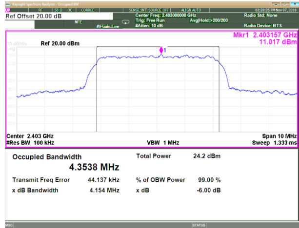
Plot 3.1.1 6 dB DTS Bandwidth, BW = 4.2 MHz, Bit rate = 1.6 Mbps, Fc = 2403MHz
