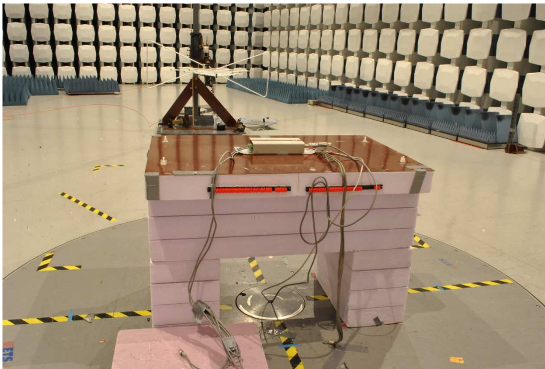
Notes: Test set-up for Radiated Emissions 30 – 2000 MHz
