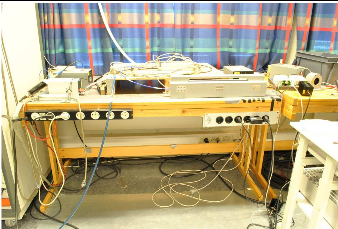
Notes: Test set-up for Conducted RF Disturbance Immunity
