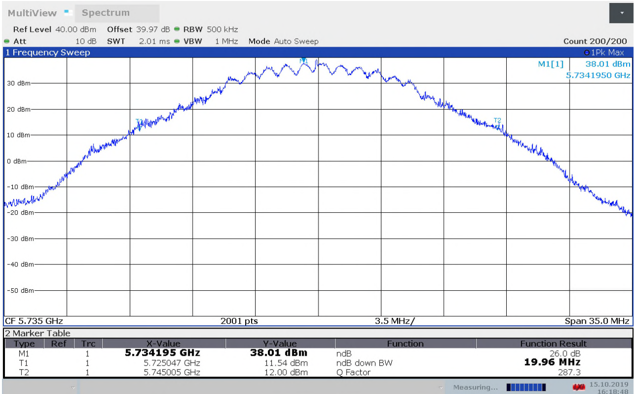
Emission Bandwidth B, 5735 MHz
