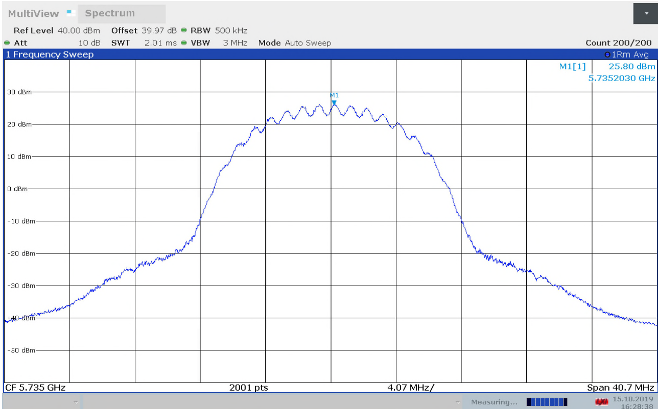
Power Spectral Density, 5735 MHz, Method 2
