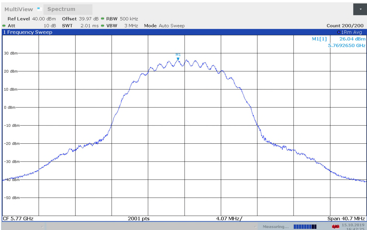
Power Spectral Density, 5770 MHz, Method 2
