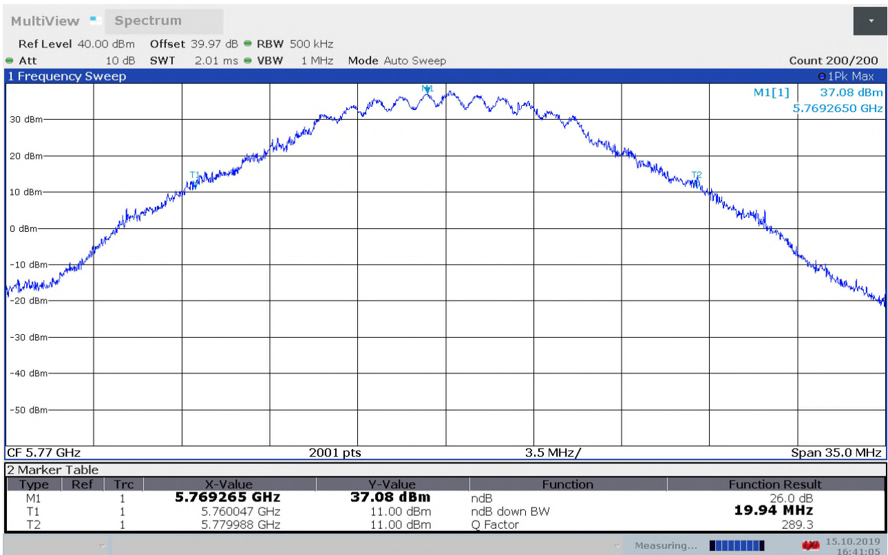
Emission Bandwidth B, 5770 MHz
