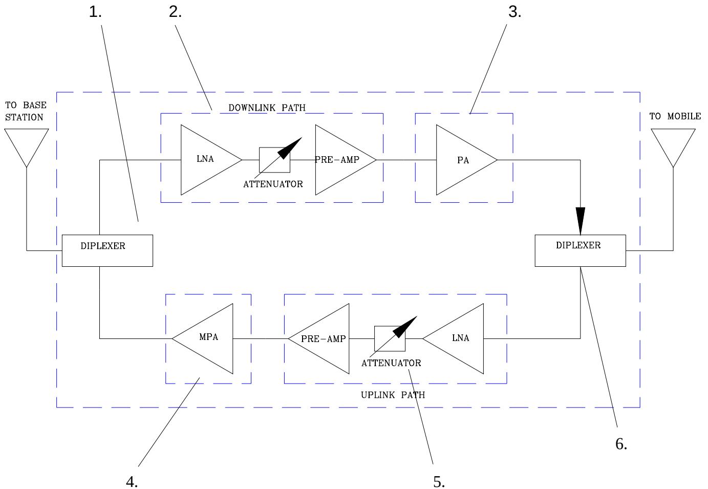
BDA BLOCK DIAGRAM BDA-XXX-1/10W-X0-A
