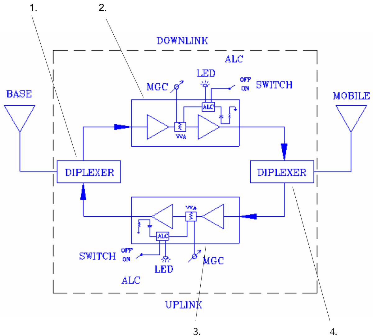
BDA BLOCK DIAGRAM BDA-XXX-1/1W-60-A
