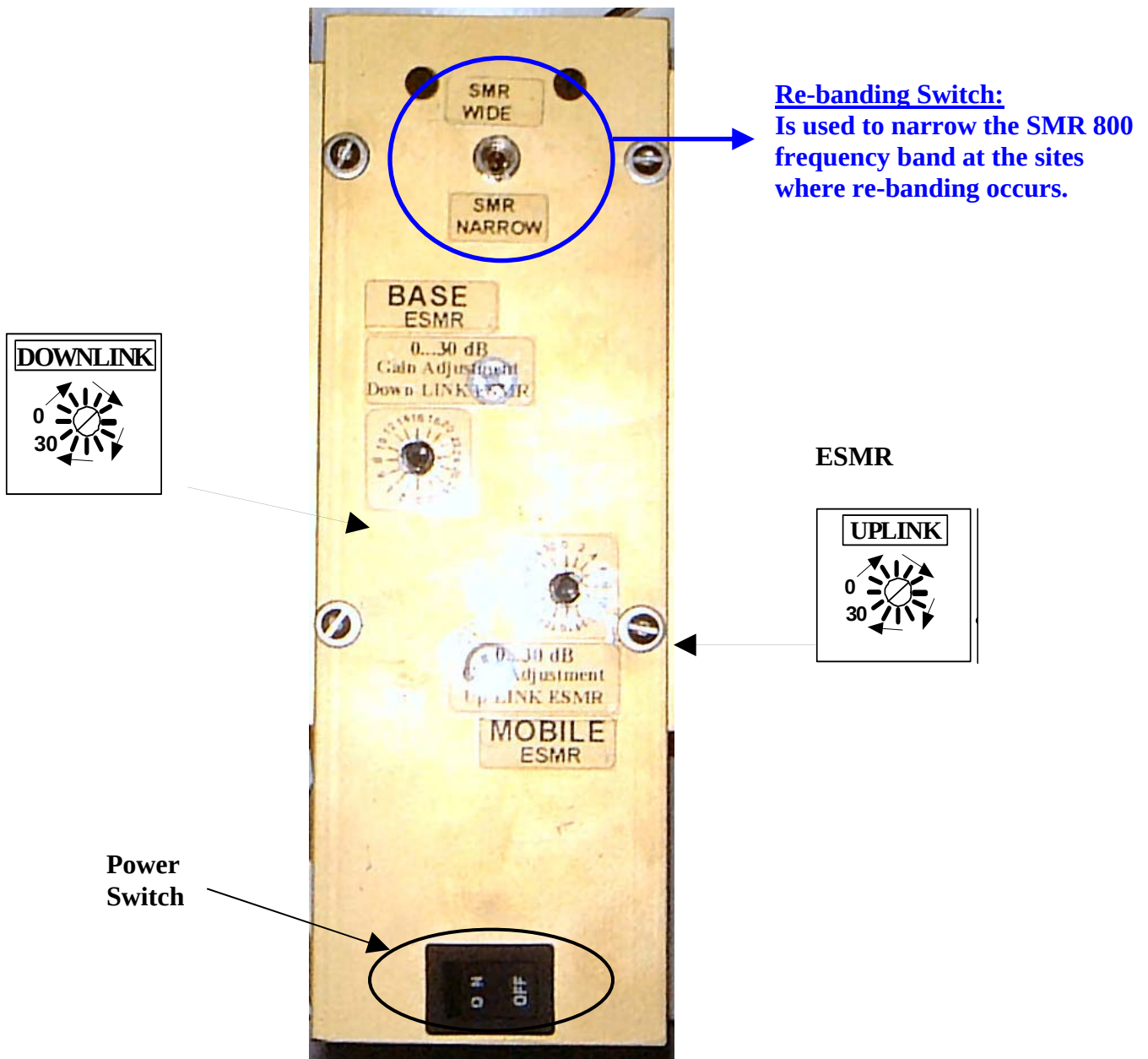
Figure 5 Control Panel
