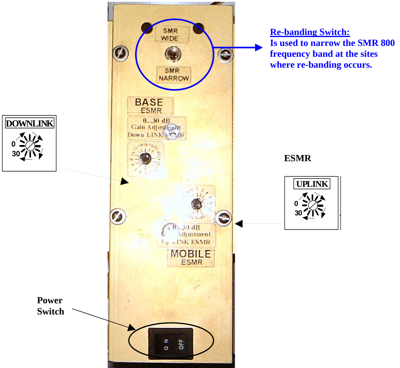
Figure 5 Control Panel
