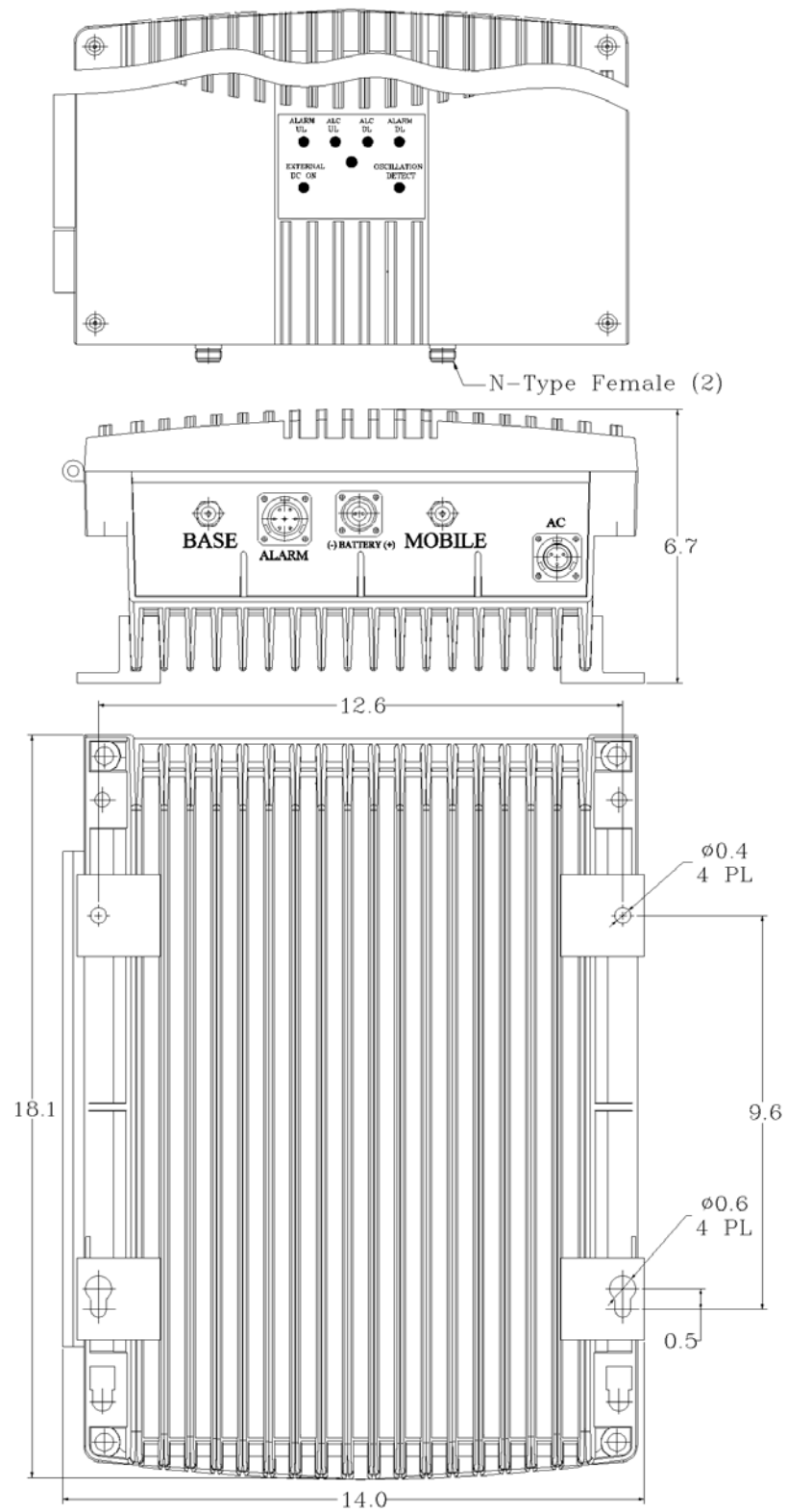
Figure 3: Mechanical Outline
