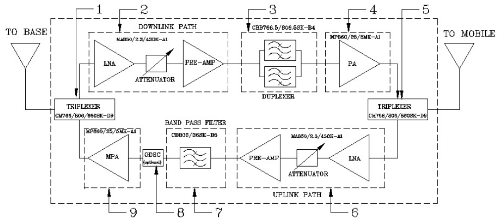
Figure 1: Block Diagram
