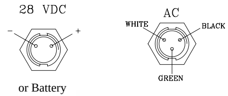
Alarm/Optional Power Supply Pinout (Relay States Refer To NON Alarm Condition)
