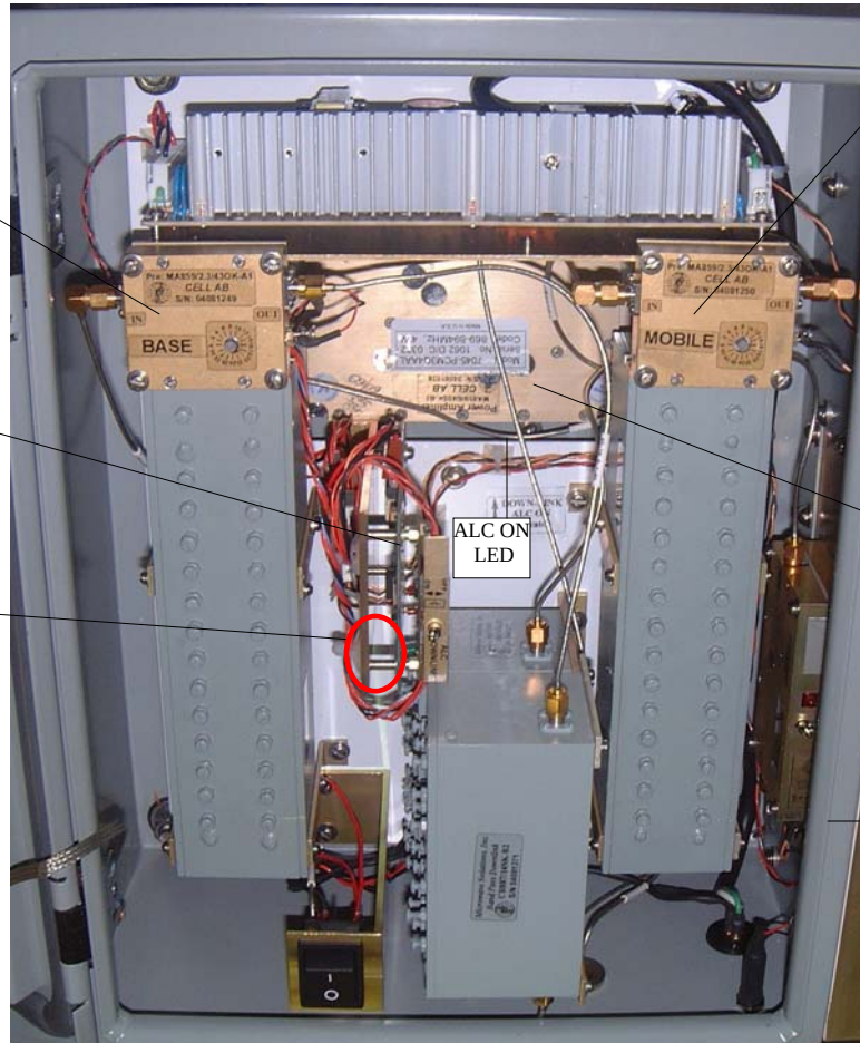
Figure 5 ALC Adjustment Access
