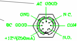
Alarm/Optional Power Supply Pinout (Relay States Refer To NON Alarm Condition)
