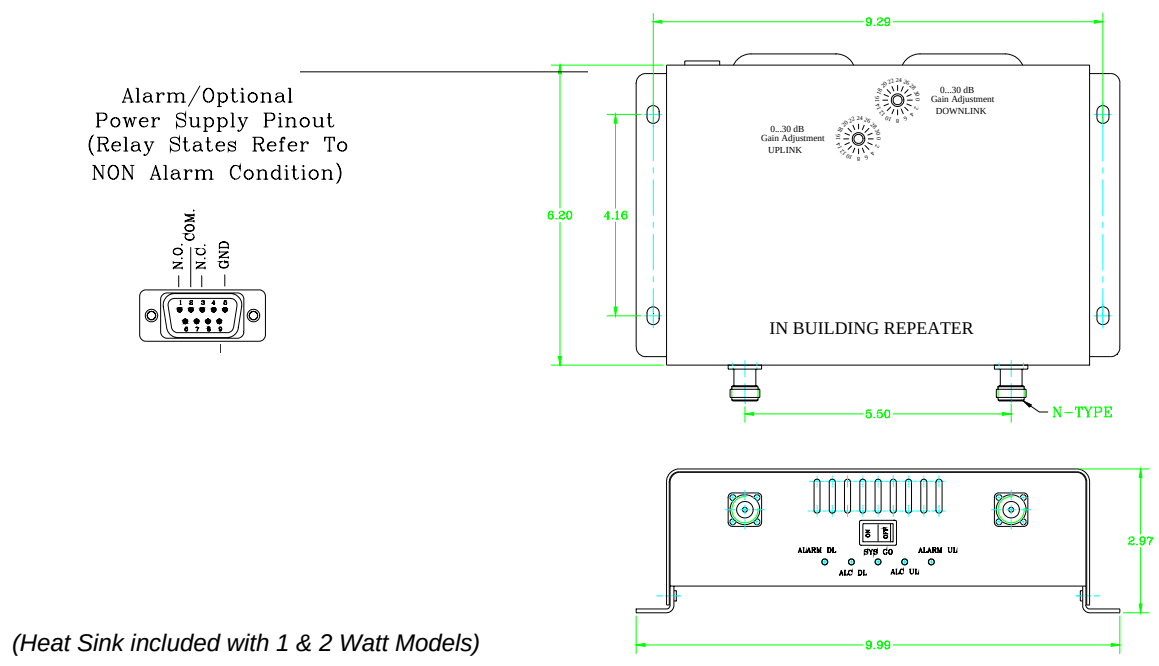
Figure 3 Mini-BDA Mechanical Outline
