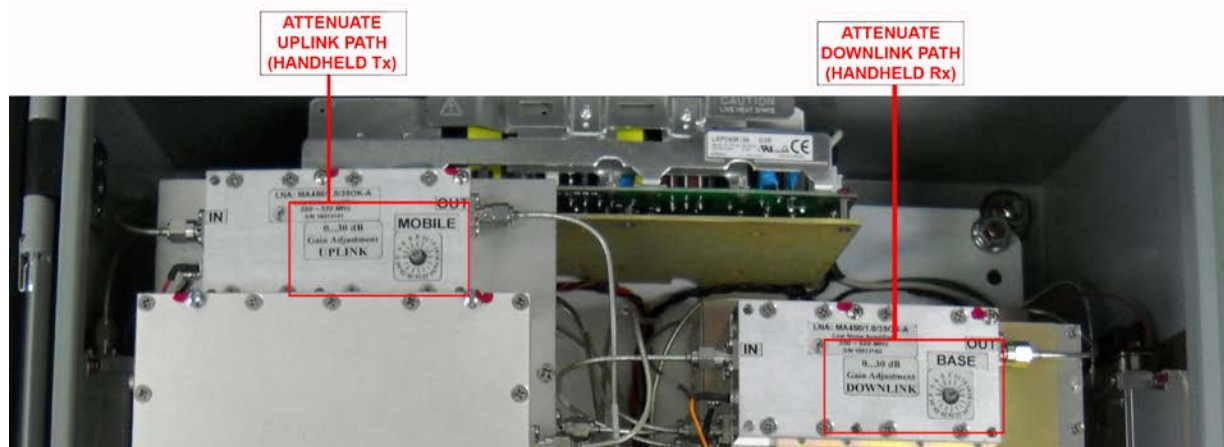
Figure 6: Manual Gain Attenuation Access Manual Gain Attenuator dials located inside the "N" Enclosure and labeled according to transmit path.
