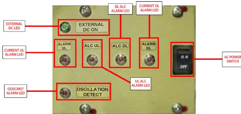
Figure 5: Internal Panel LED Indication
