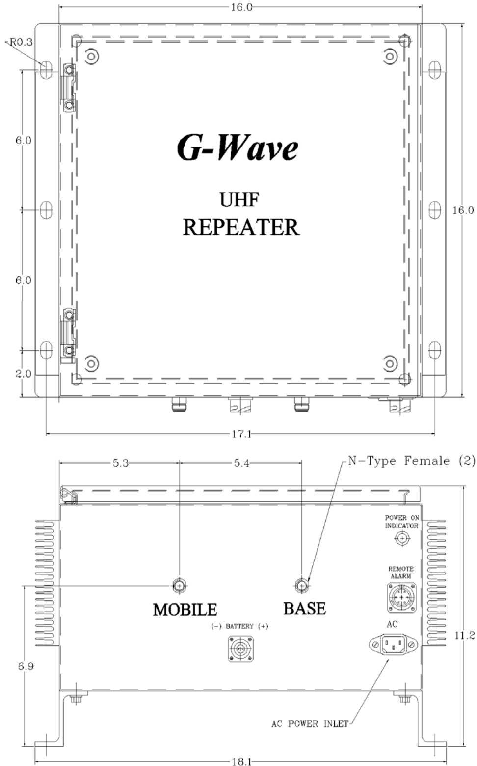
Figure 3: Mechanical Outline
