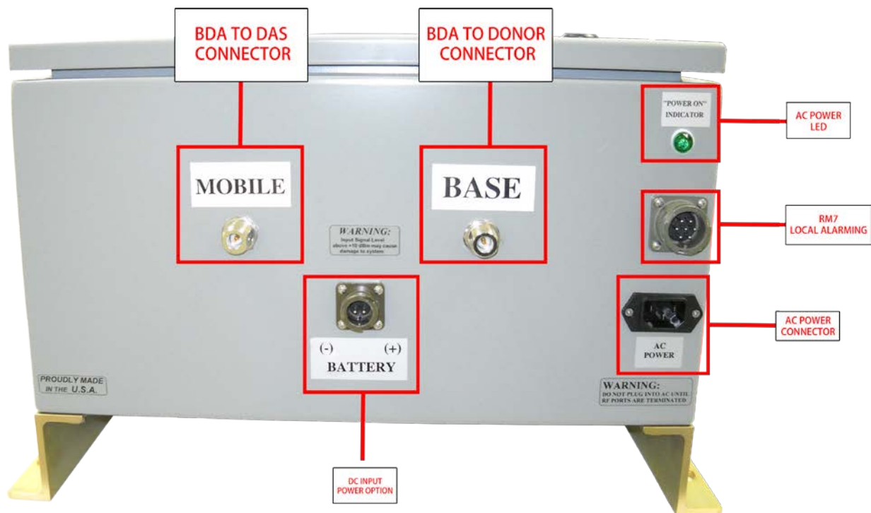
Figure 4: Front Panel Connections
