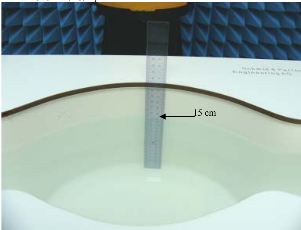
Fig.9 Photograph of the Tissue Simulant Fluid liquid depth 15cm
