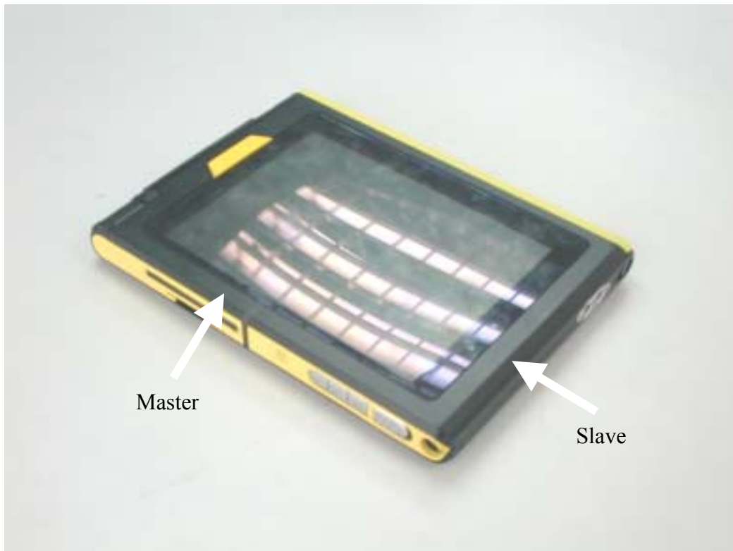
Fig.12 Photograph of the Tablet Pc that Master and Slave 802.11b antennas are identical and the Master antenna is used for SAR measurement
