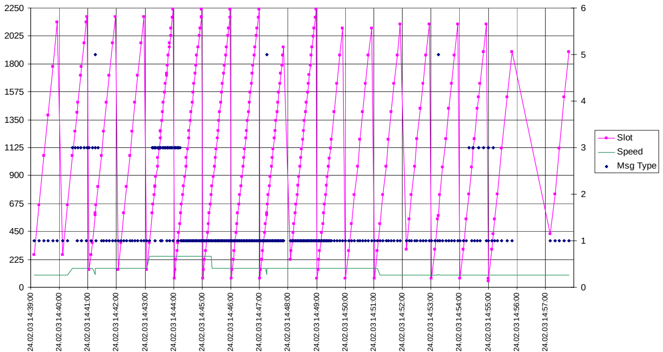
24.02.03 - 14.4.1 - Nauticast X-Pack DS - Reporting rate by speed - Slot offset
