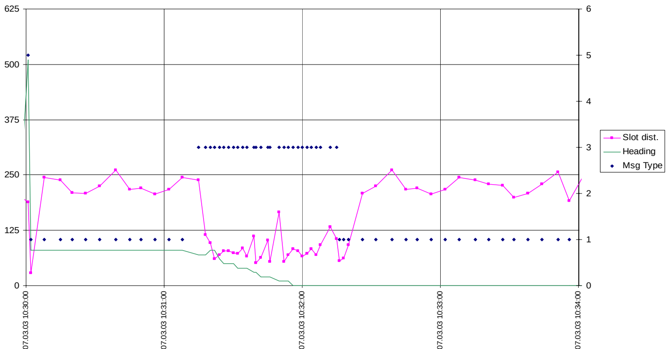
07.03.03 Nauticast X-Pack DS - 14.4.1 - Reporting rate change by heading at 15 kn - Slot offset
