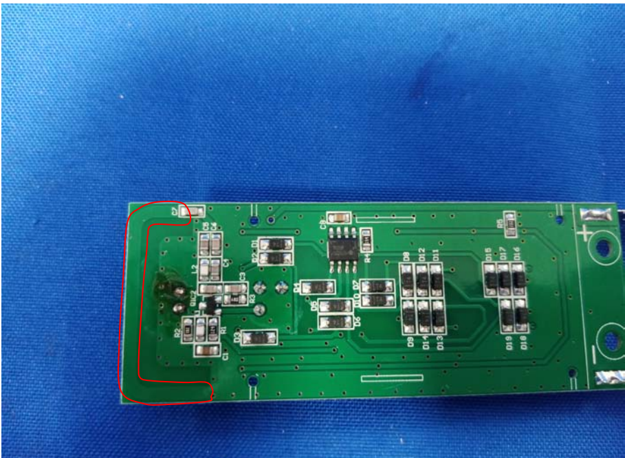
433.92MHz TX Antenna
