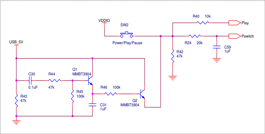
Play Switch Circuit /w auto power-up (MS mode)
