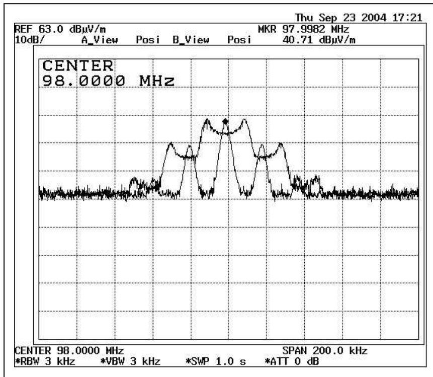
Bandwidth 2 – 98.0 MHz
