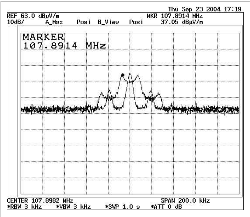
Bandwidth 3 – 107.9 MHz
