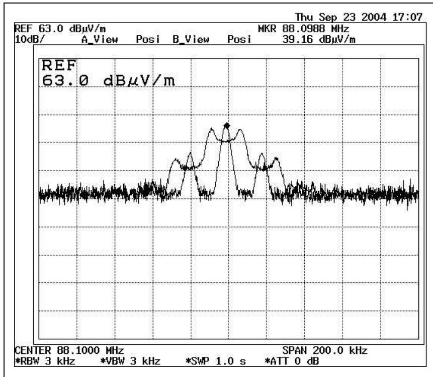
Bandwidth 1 – 88.1 MHz
