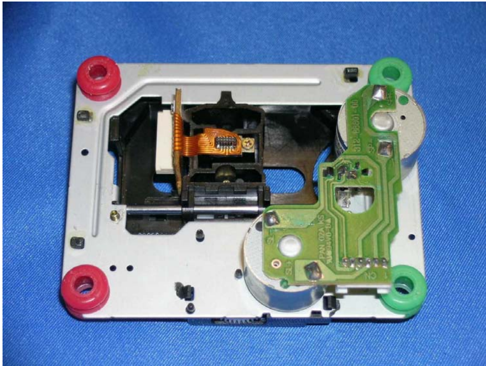
CD loader rear side (View 1)
