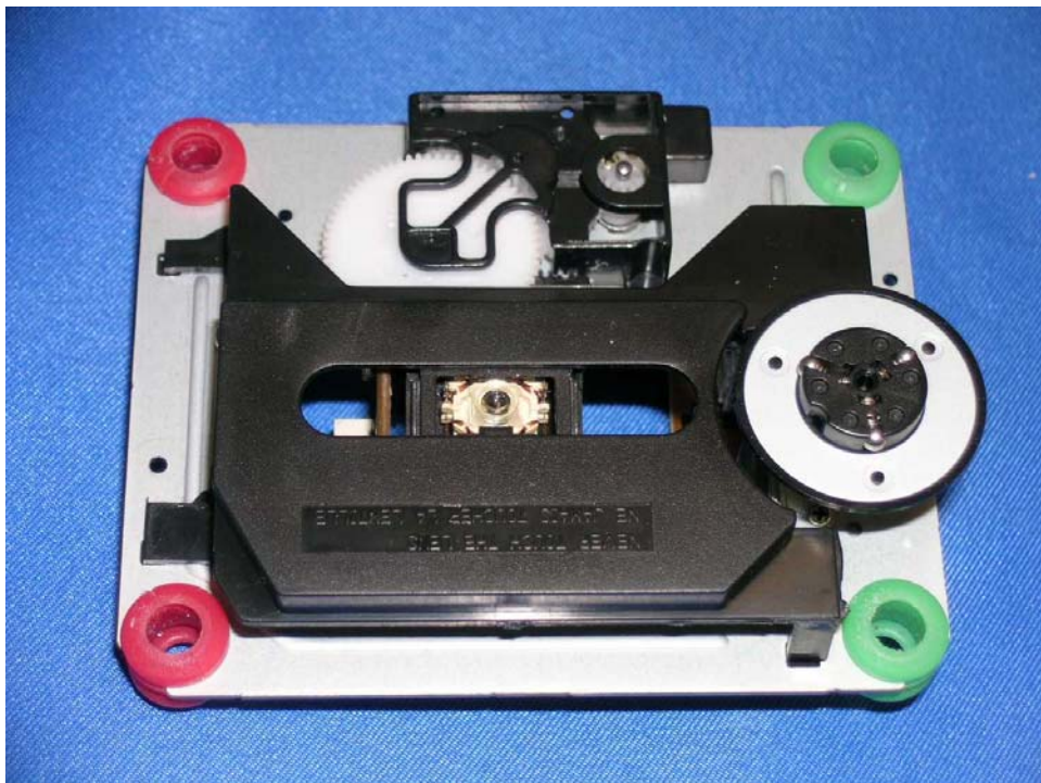
CD loader front side
