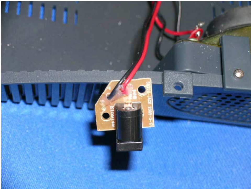
AC Power Jack front side
