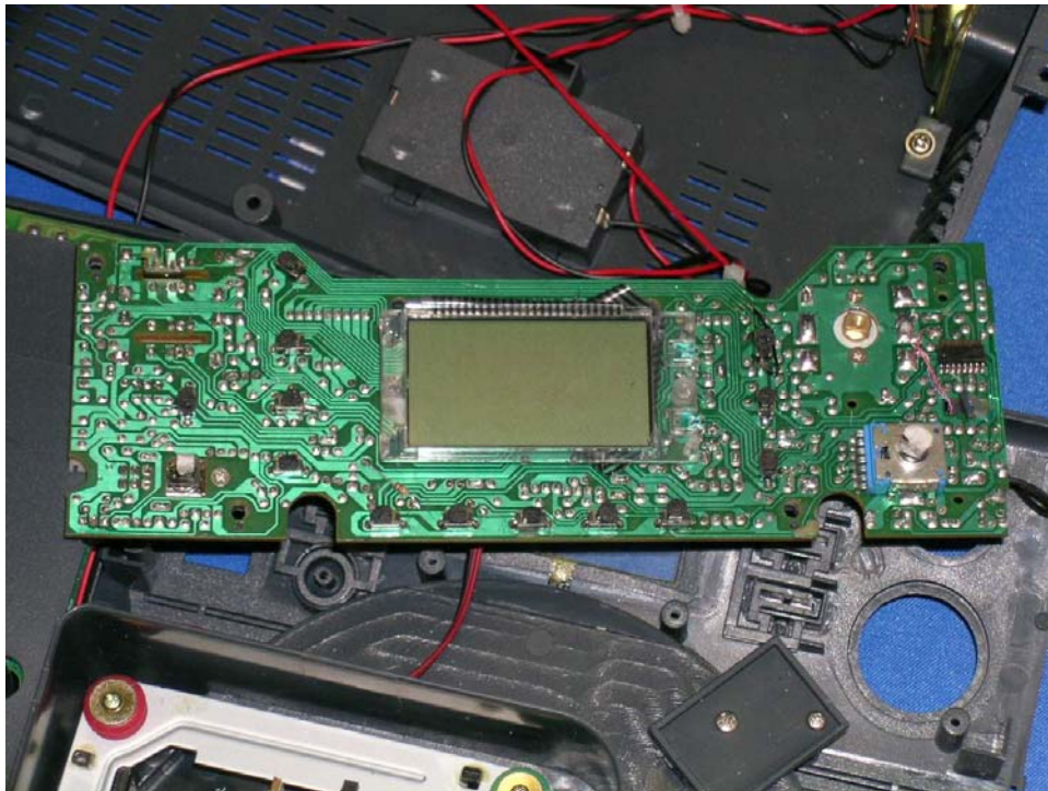
LCD display front side
