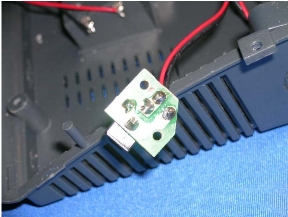
AC Power Jack rear side
