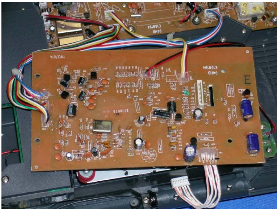
CD Player PCB comp side
