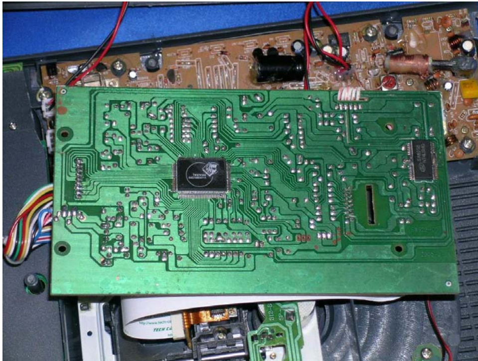
CD Player PCB solder side
