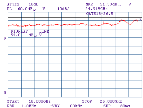
Plot 7.7.30 Radiated emission measurements from 18.0 to 25.0 GHz at the high carrier frequency
