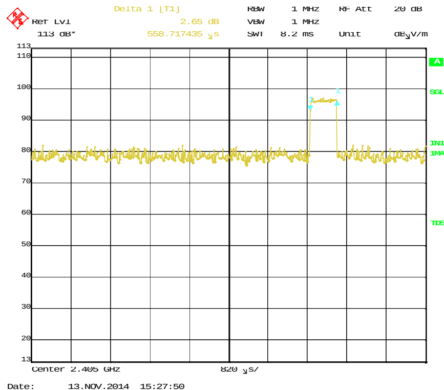
Figure 33. Burst Duration
