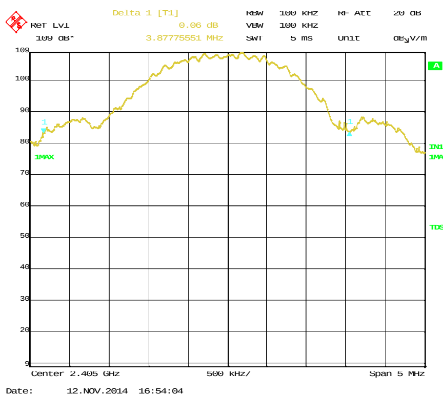
Figure 13 — 2405 MHz Channel
