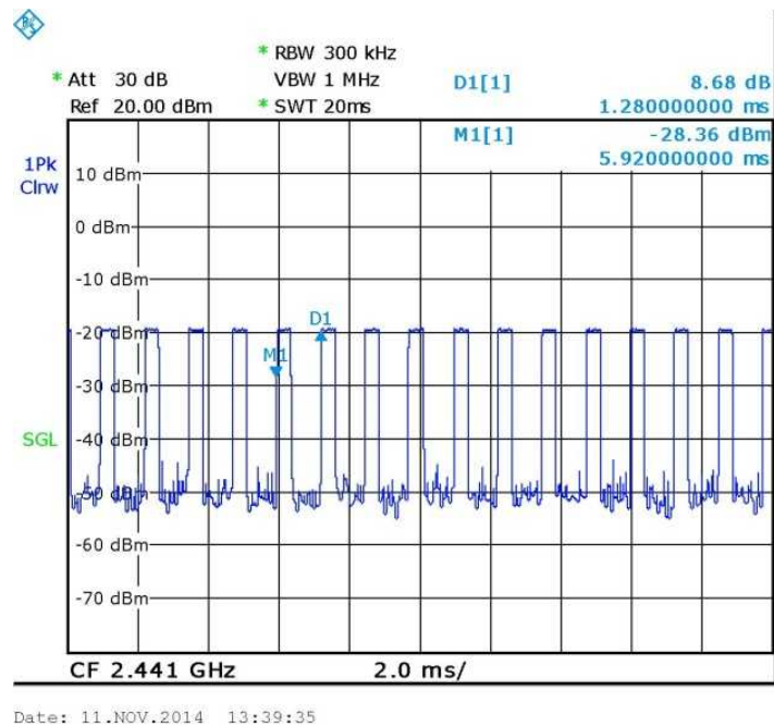
Figure 11. Number of bursts in 20msec=16 Number of bursts in 100msec=80
