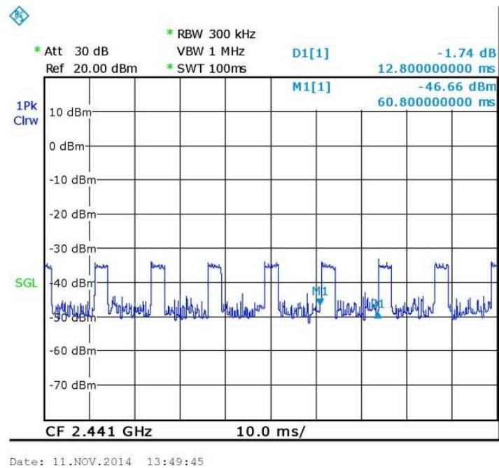
Figure 13. Number of bursts in 100msec=9
