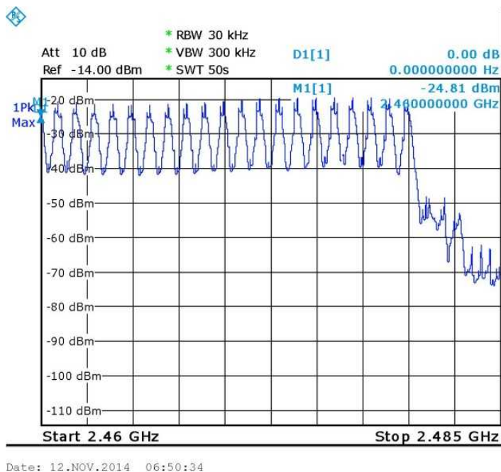
Figure 32. Frequency Hopping, Standard modulation
