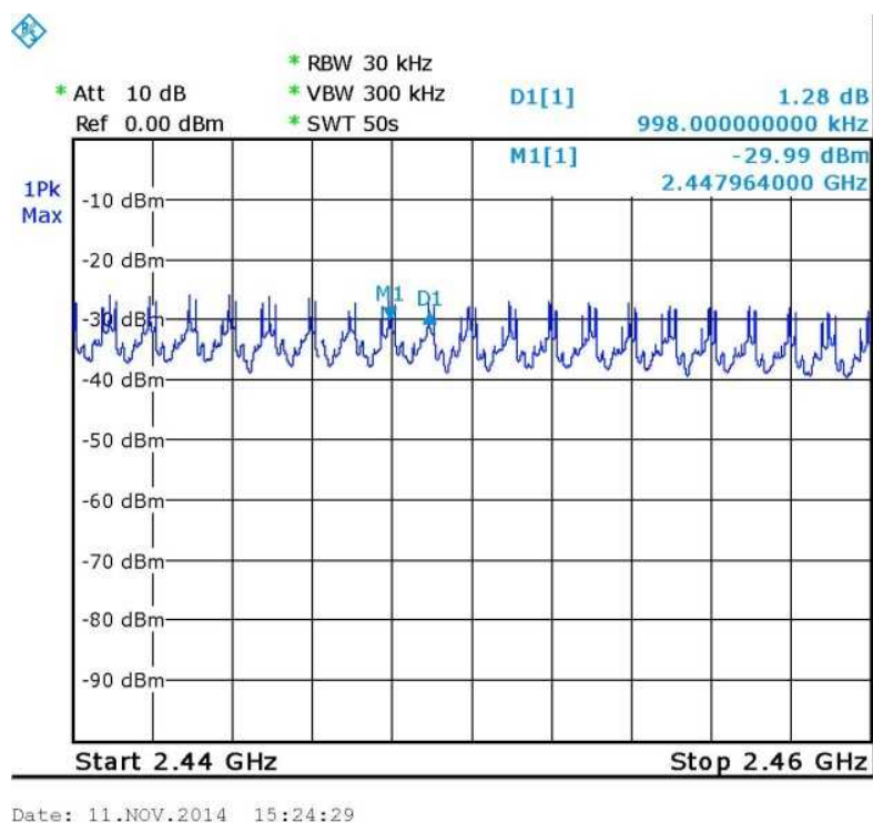
Figure 40. EDR Modulation
