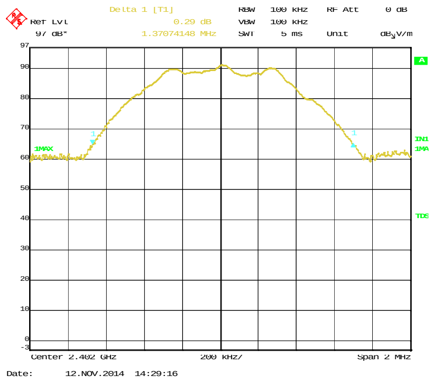
Figure 17. Low Channel, BLE Modulation
