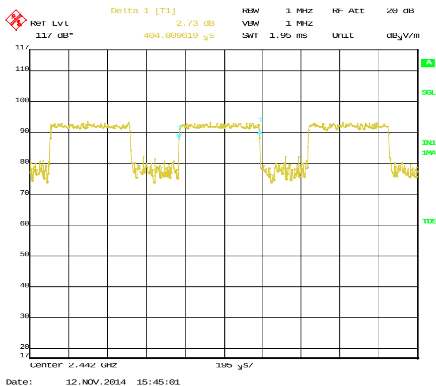
Figure 10. Burst Duration
