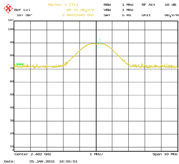
Figure 23 2402.00 MHz – Horizontal, BLE Modulation
