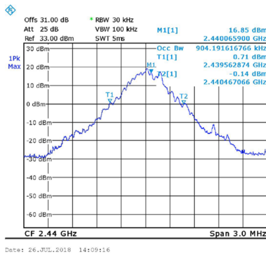
Figure 10. STD, Mid
