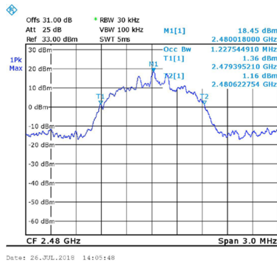
Figure 14. EDR, High
