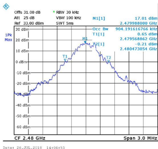
Figure 11. STD, High
