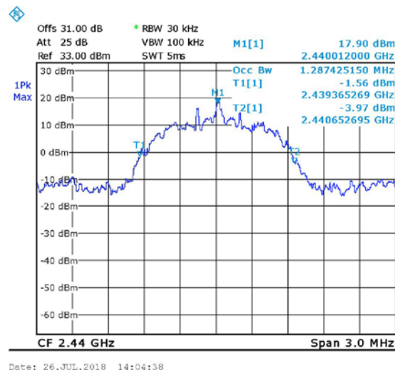
Figure 13. EDR, Mid
