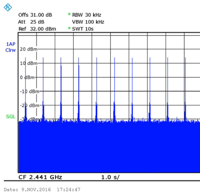
Figure 23 — Number of Bursts in 10 sec=10 EDR modulation
