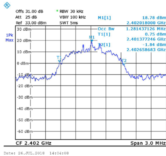
Figure 12. EDR, Low
