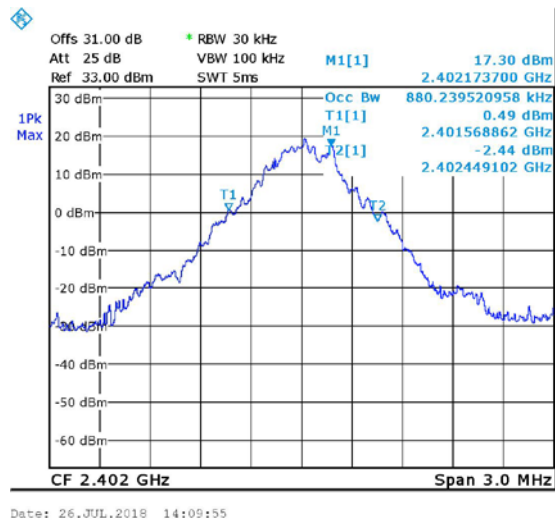
Figure 9. STD, Low
