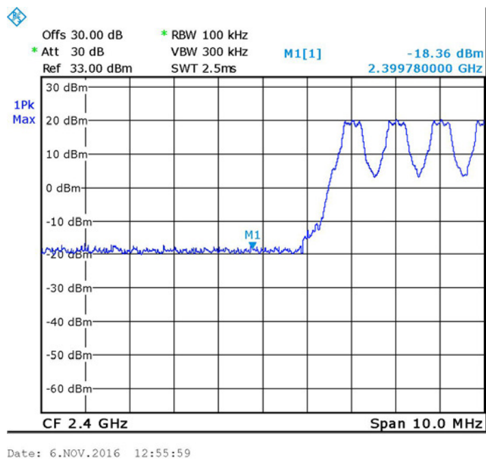
Figure 60 — Hopping - Low Standard Modulation
