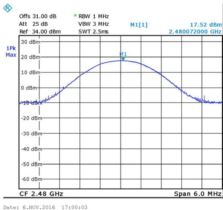
Figure 52 — 2480MHz - High EDR Modulation
