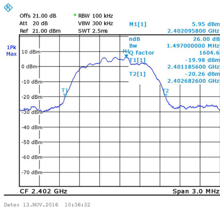
Figure 28. —2402 MHz - Low - EDR Modulation
