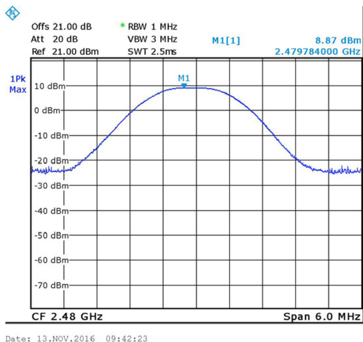
Figure 49 — 2480MHz - High - Standard Modulation
