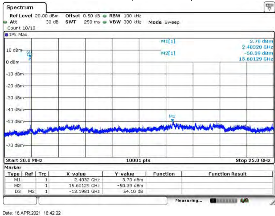
Channel 00 (30MHz-25GHz)
