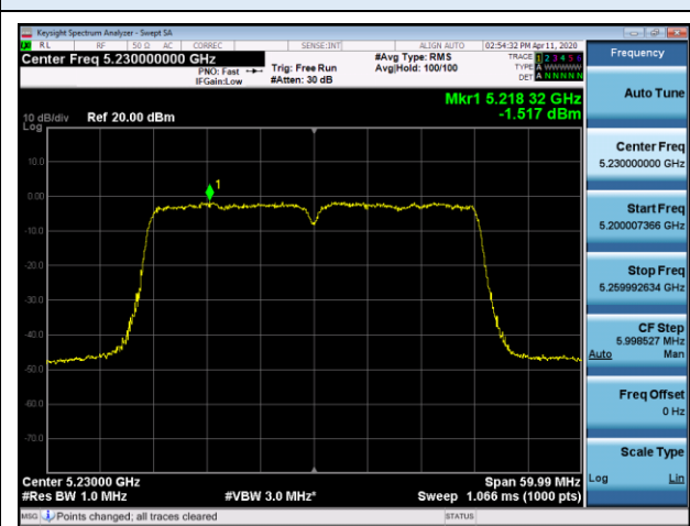
802.11ac VHT40 UNII 1 BAND PSD (CH 46)
