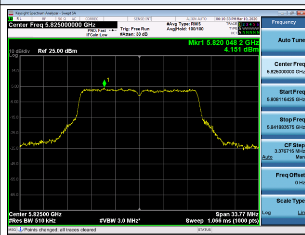
802.11a UNII 3 BAND PSD (CH 165)
