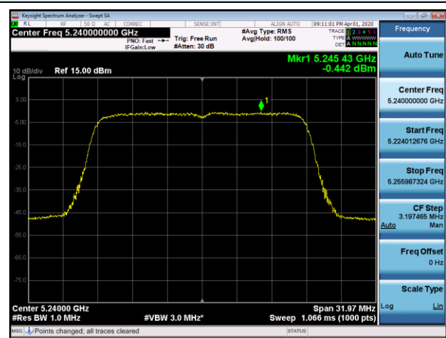
802.11ax HE20 UNII 1 BAND PSD (CH 48)
