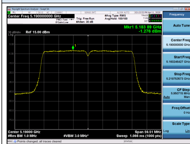
802.11ac VHT40 UNII 1 BAND PSD (CH 38)
