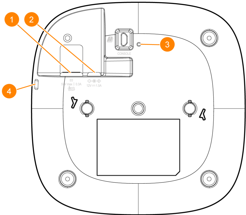
Figure 2 Rear View
