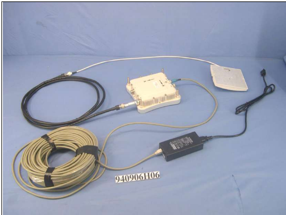
EUT with Antenna Model No.: AP-ANT-81
