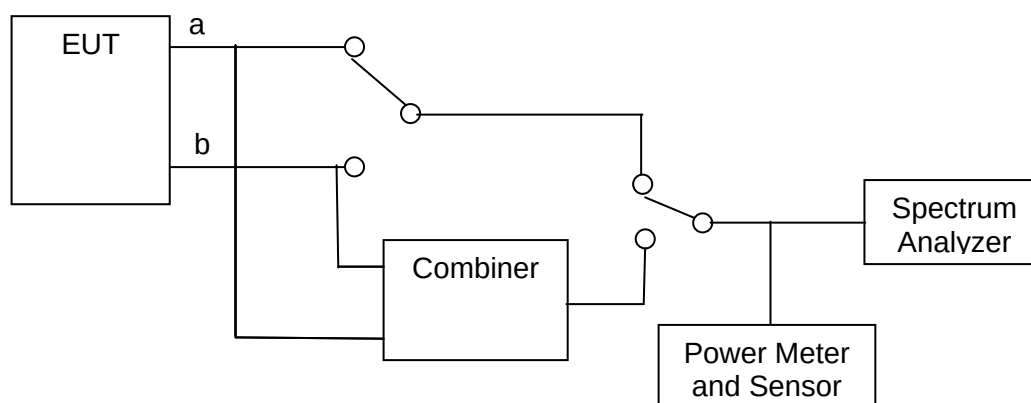
Measurement set up for Peak Excursion Ratio
