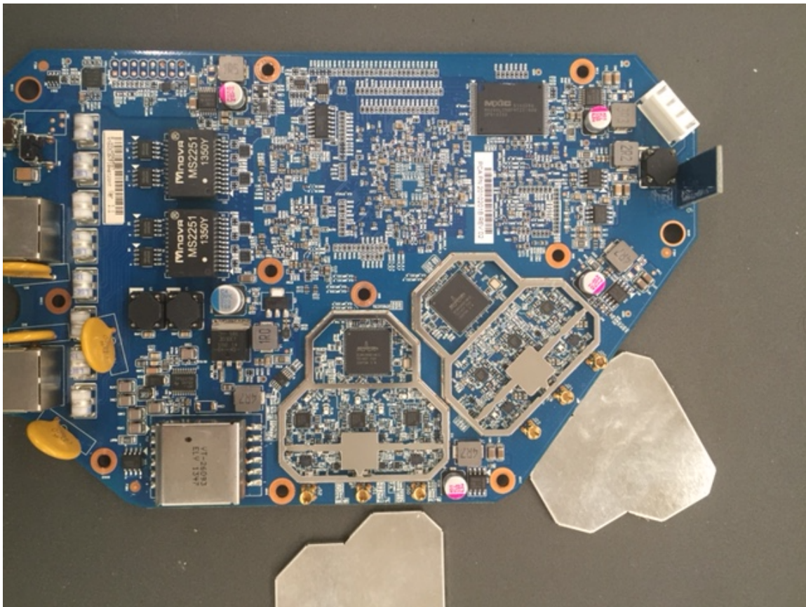
RF Board Top View with Shields Removed
