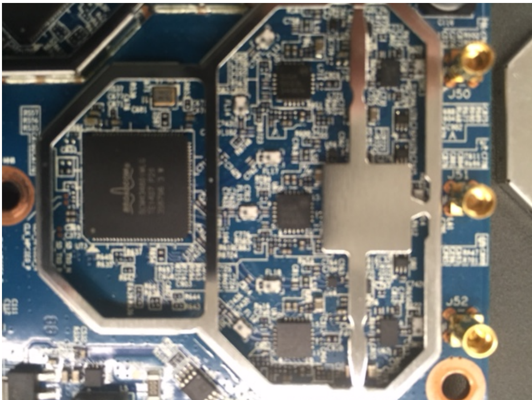
5GHz RF Board Close-Up
