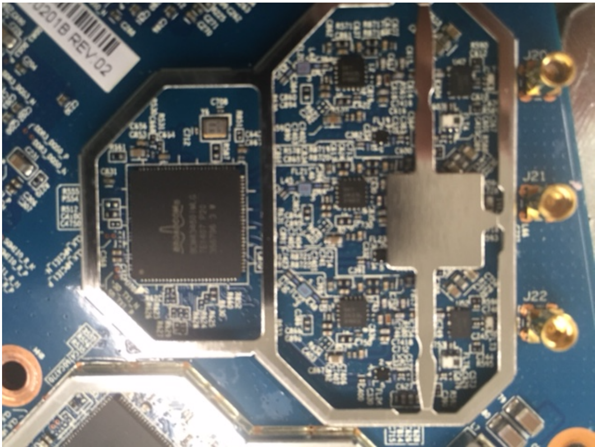
2.4GHz RF Board Close-Up
