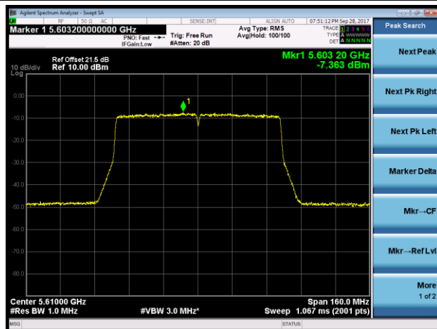
Channel 122 (5610MHz)
