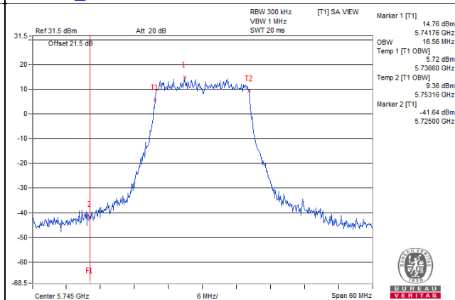
802.11ac(VHT20)_Chain1 / CH149
