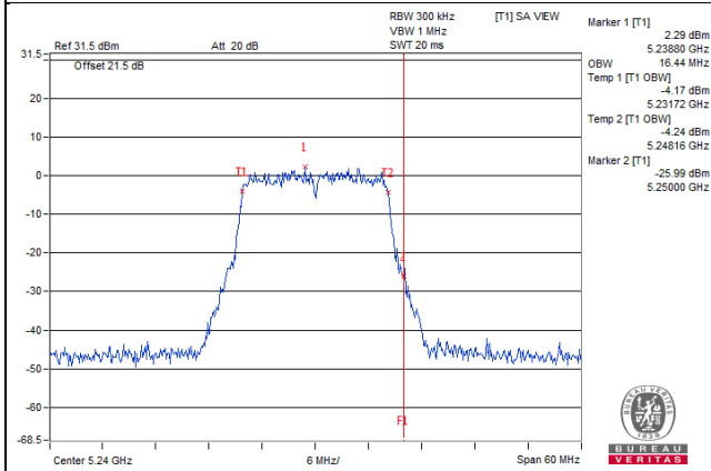
802.11ac(VHT20)_Chain0 / CH48
