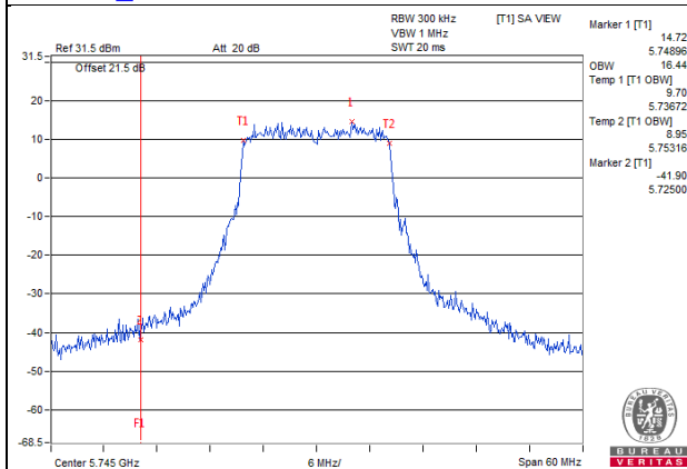
802.11ac(VHT20)_Chain0 / CH149
