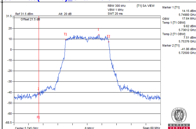
802.11ac(VHT20)_Chain1 / CH149
