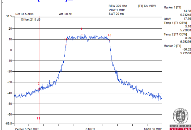
802.11ac(VHT20)_Chain0 / CH149
