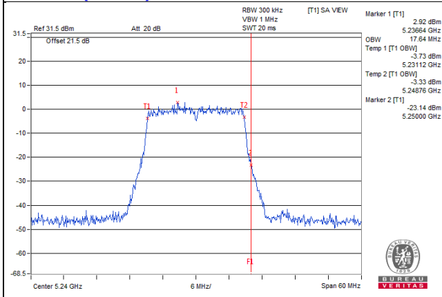
802.11ac(VHT20)_Chain0 / CH48
