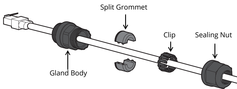
Figure 2 Installing the Ethernet Cable Gland
