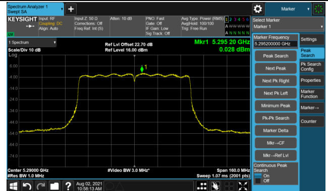
Channel 58 (5290MHz)
