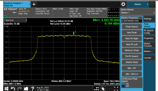
Channel 58 (5290MHz)
