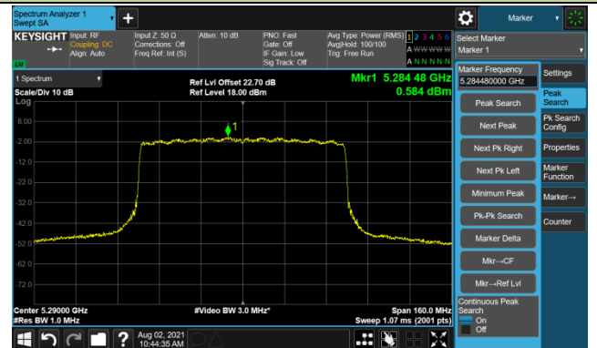
Channel 58 (5290MHz)
