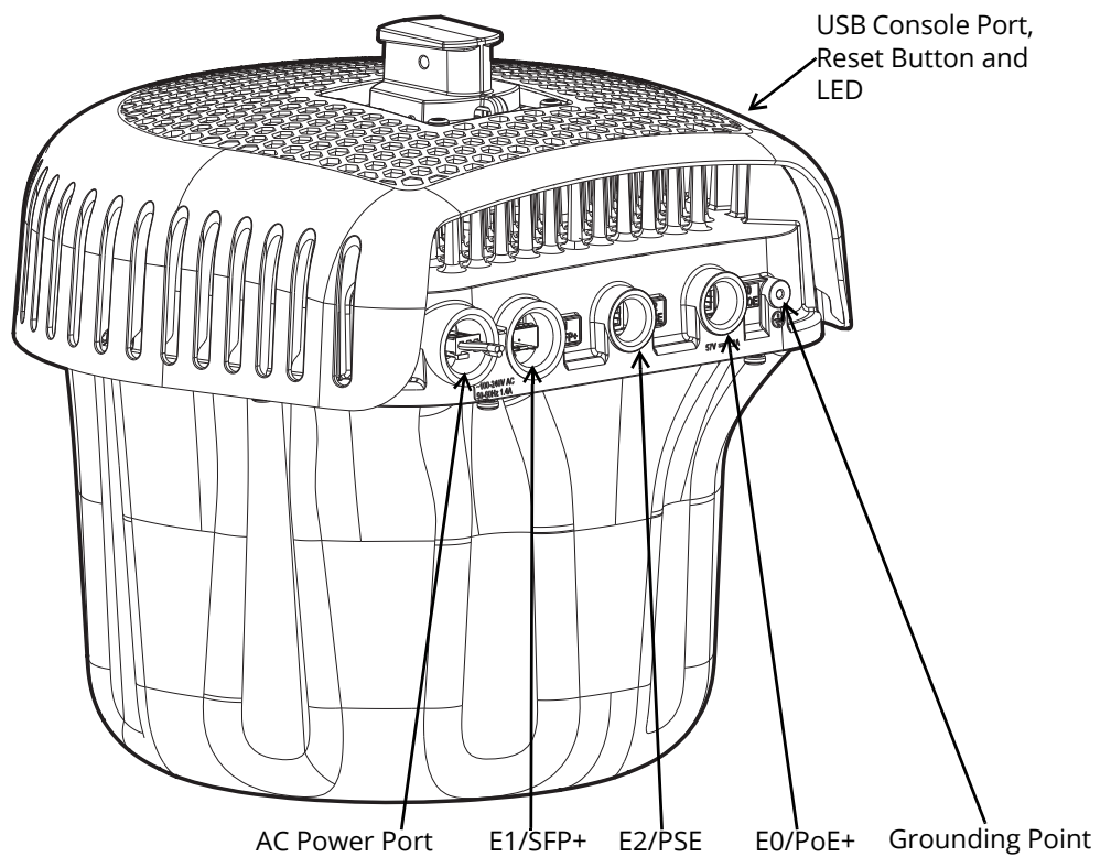
Figure 4 AP-585 Rear View
