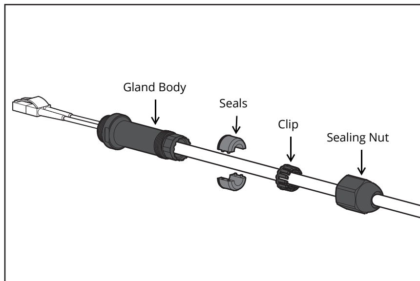
Figure 10 Fiber-optic Cable and CKIT-OD-SFP SFP Cable Gland
