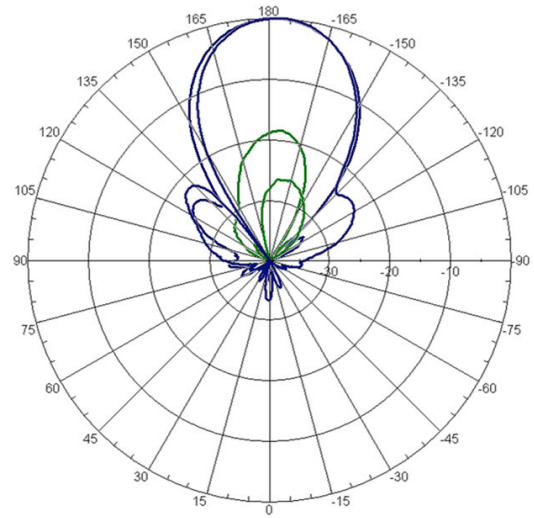
Horizontal Pattern
