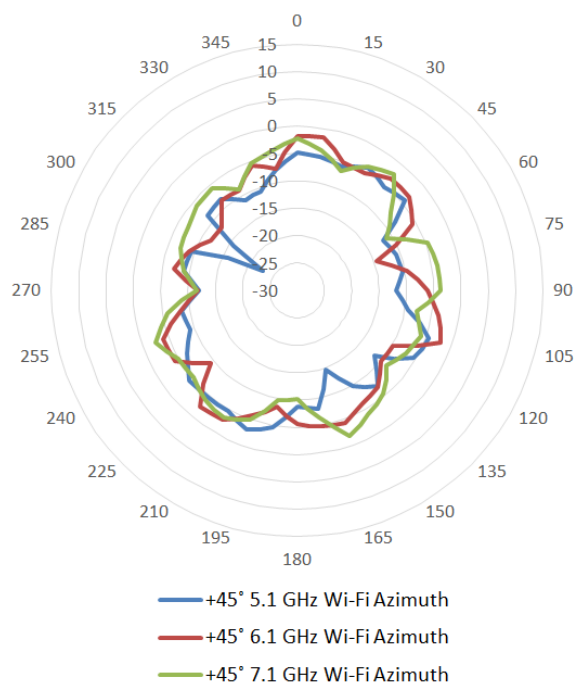
+45° antenna patterns (Azimuth)
