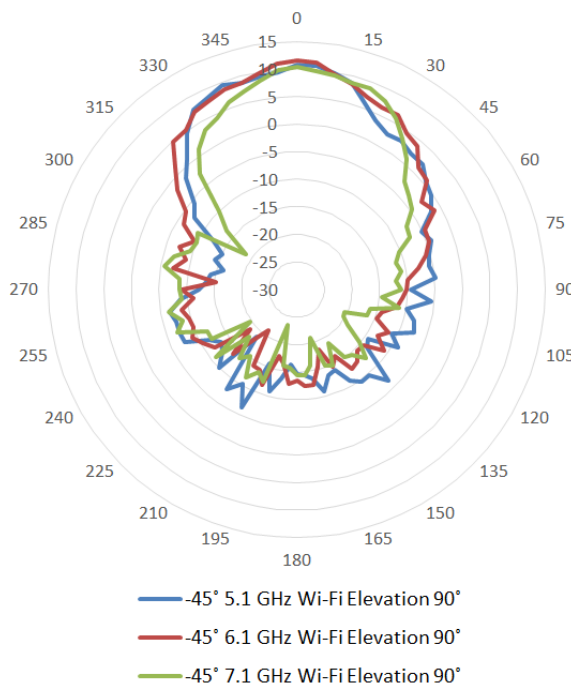
-45° antenna patterns (Elevation 90°)
