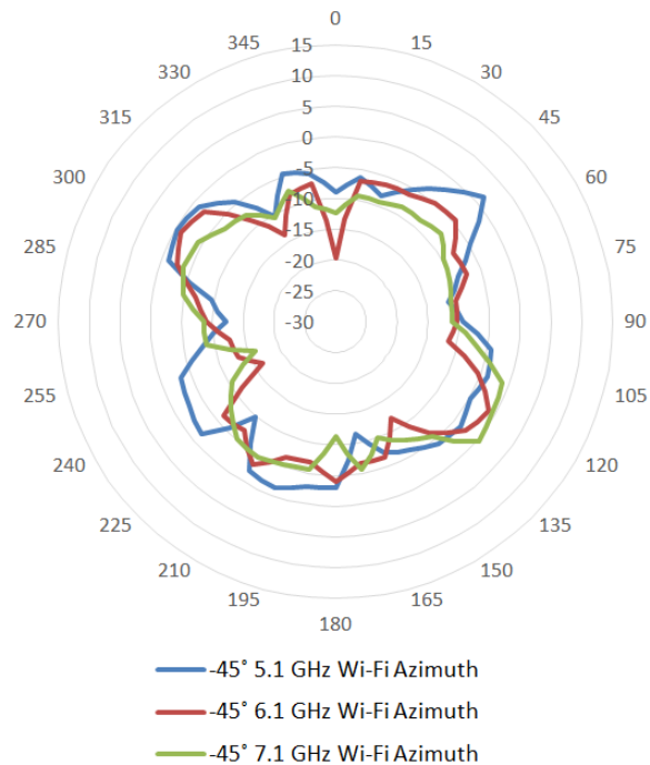
-45° antenna patterns (Azimuth)
