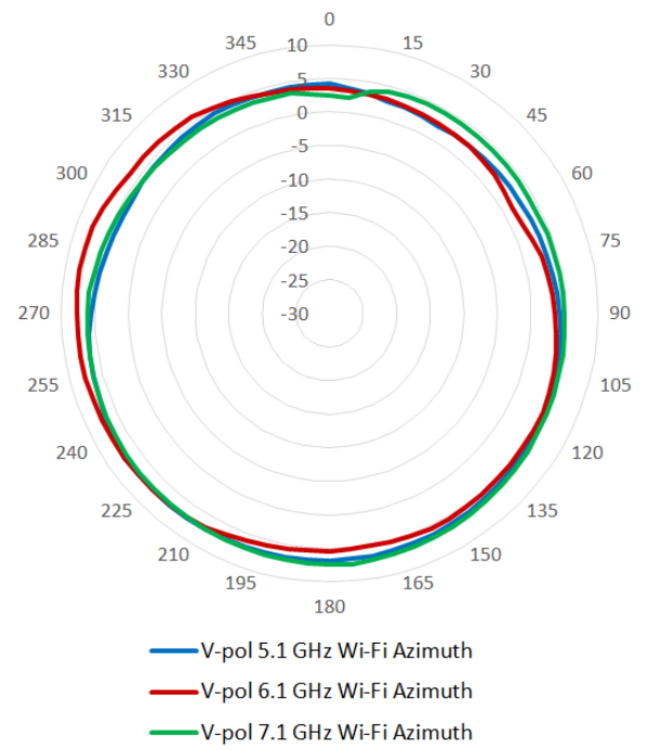
V-pol antenna patterns (Azimuth)
