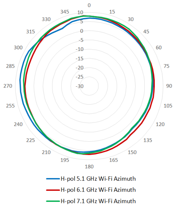
H-pol antenna patterns (Azimuth)
