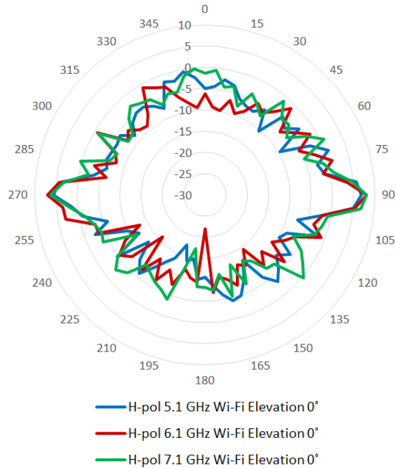
H-pol antenna patterns (Elevation 0°)
