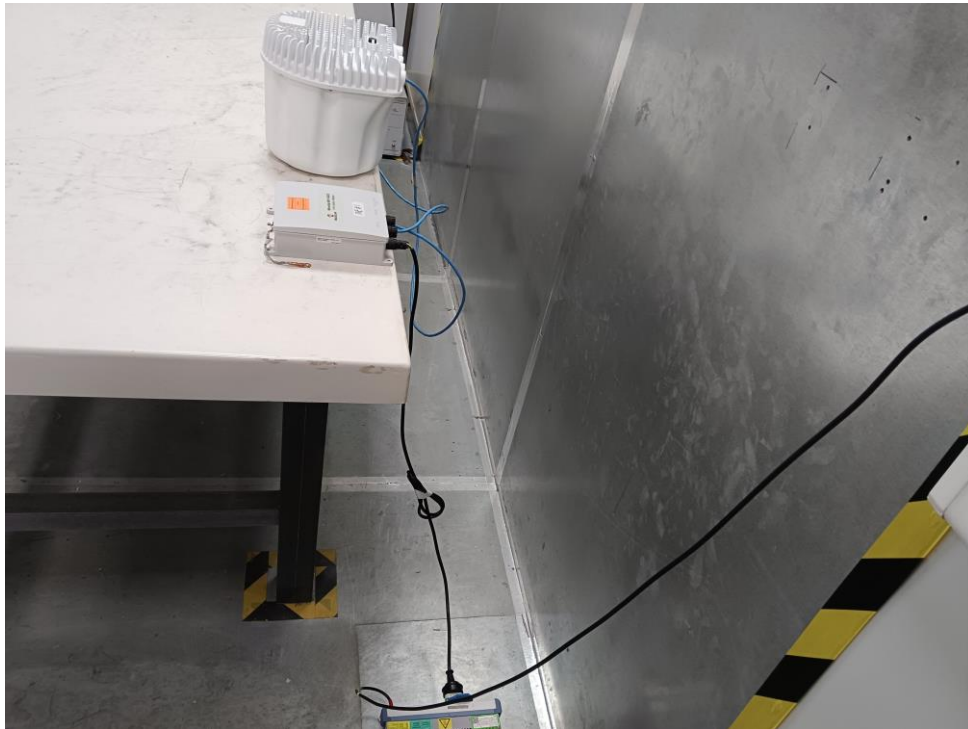
Description: Back View of Conducted Emission Test Setup - APEX0675
