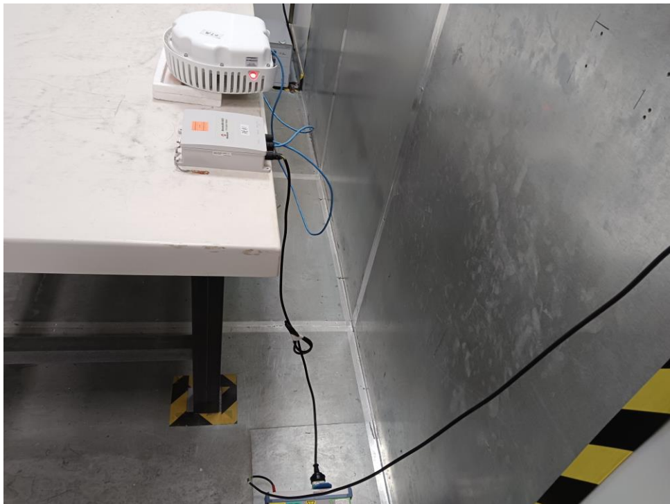
Description: Back View of Conducted Emission Test Setup - APEX0679
