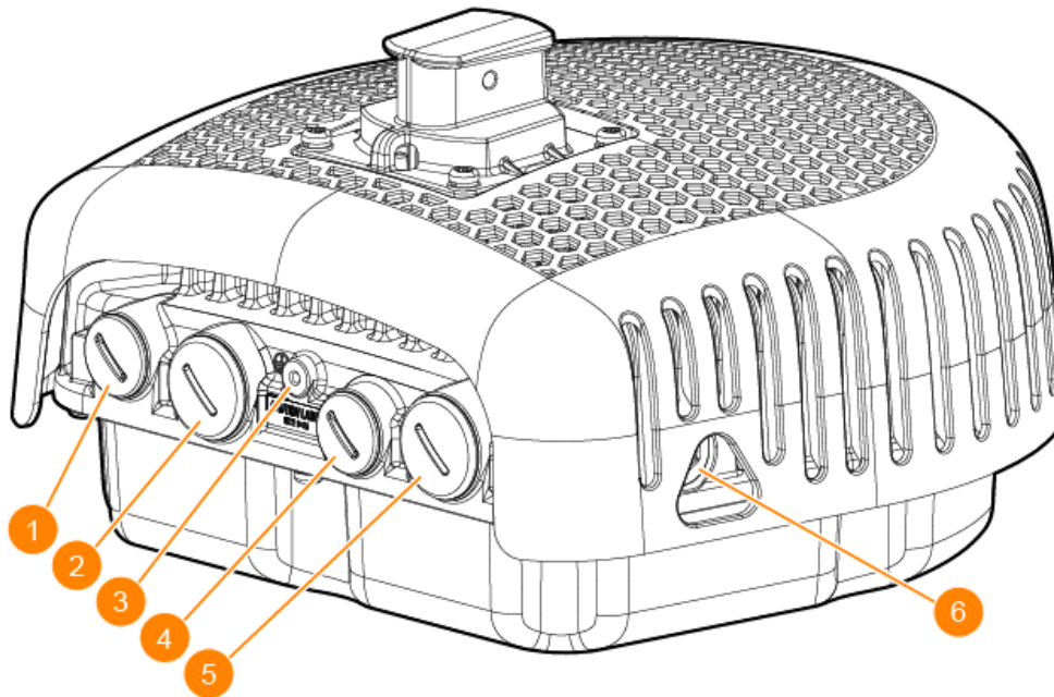
Figure 6 AP-677/AP-679 Back View
