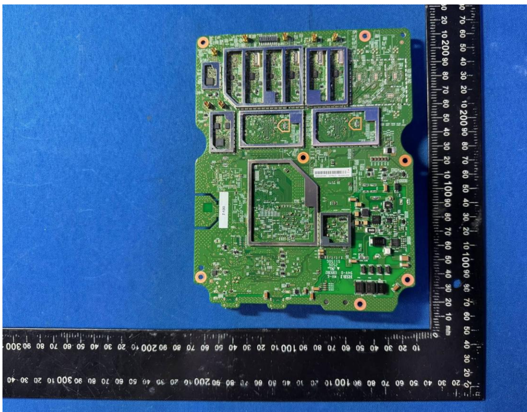
(38) EUT Photo
