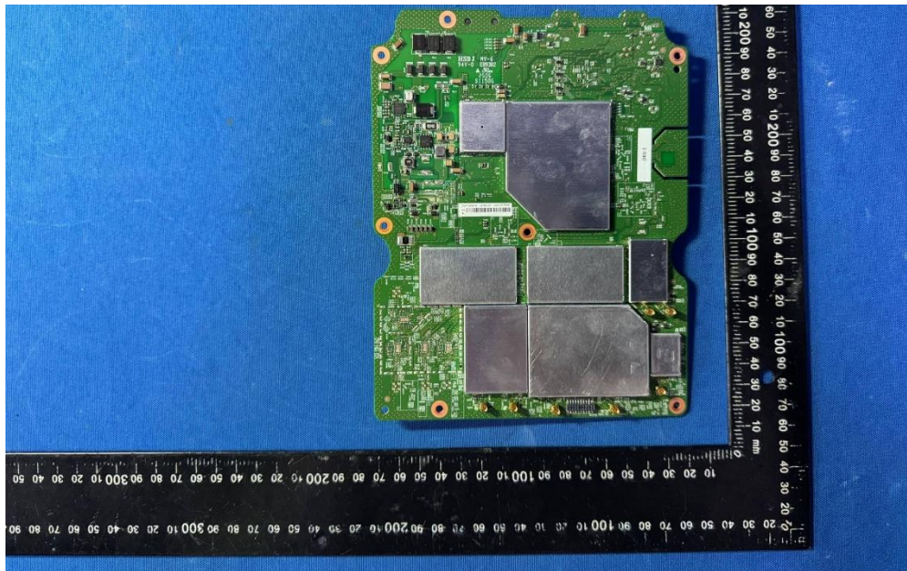
(28) EUT Photo
